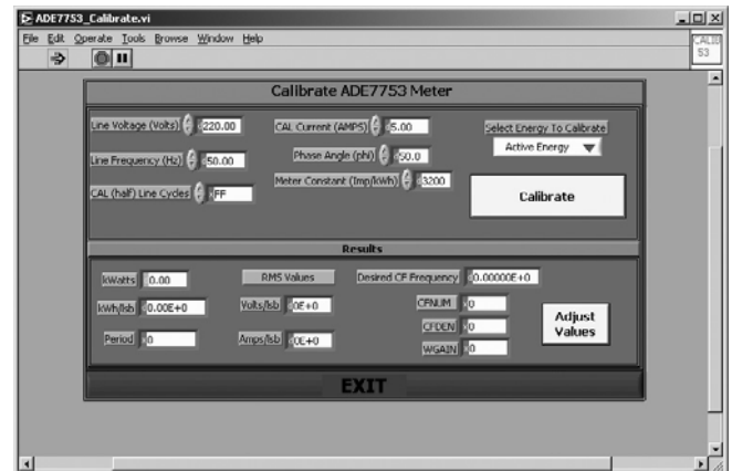
Figure 11. Calibration Window
