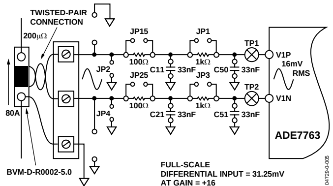
Figure 5. Shunt Connection to Current Channel
