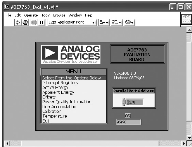
Figure 10. Main Menu
