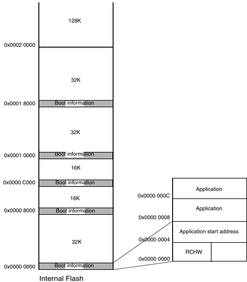
Figure 481. SPC560P40/34 Flash partitioning and RCHW search
