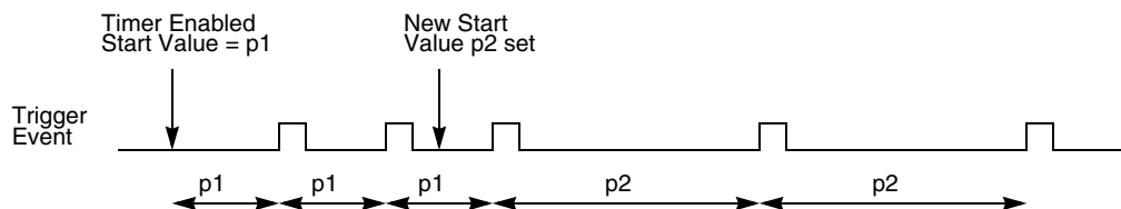
Figure 464. Dynamically setting a new load value
