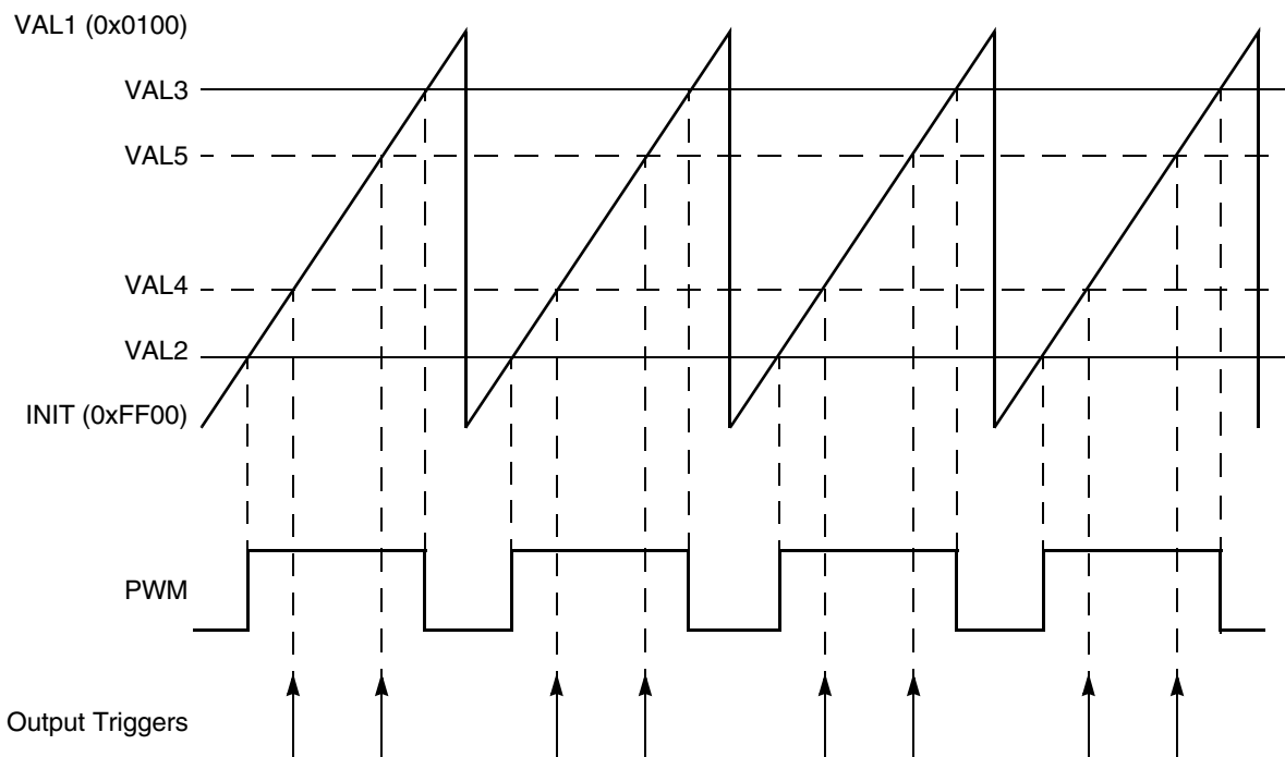
Figure 366. Multiple output trigger generation in hardware
