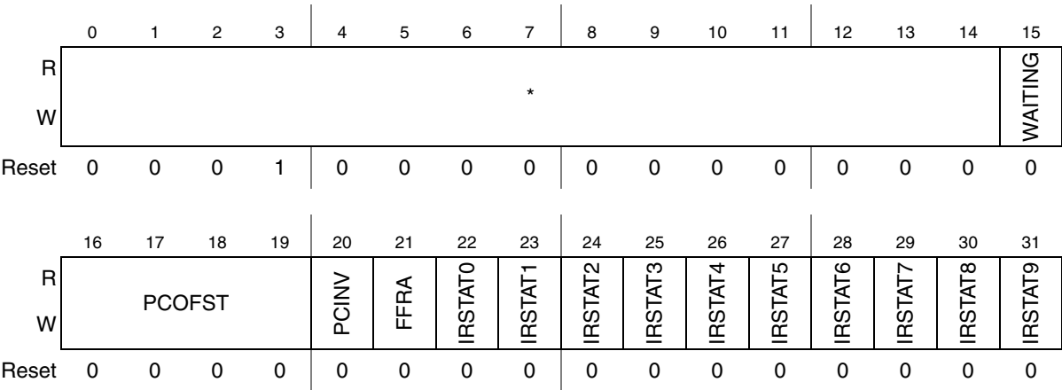
Figure 520. Control State Register (CTL)
