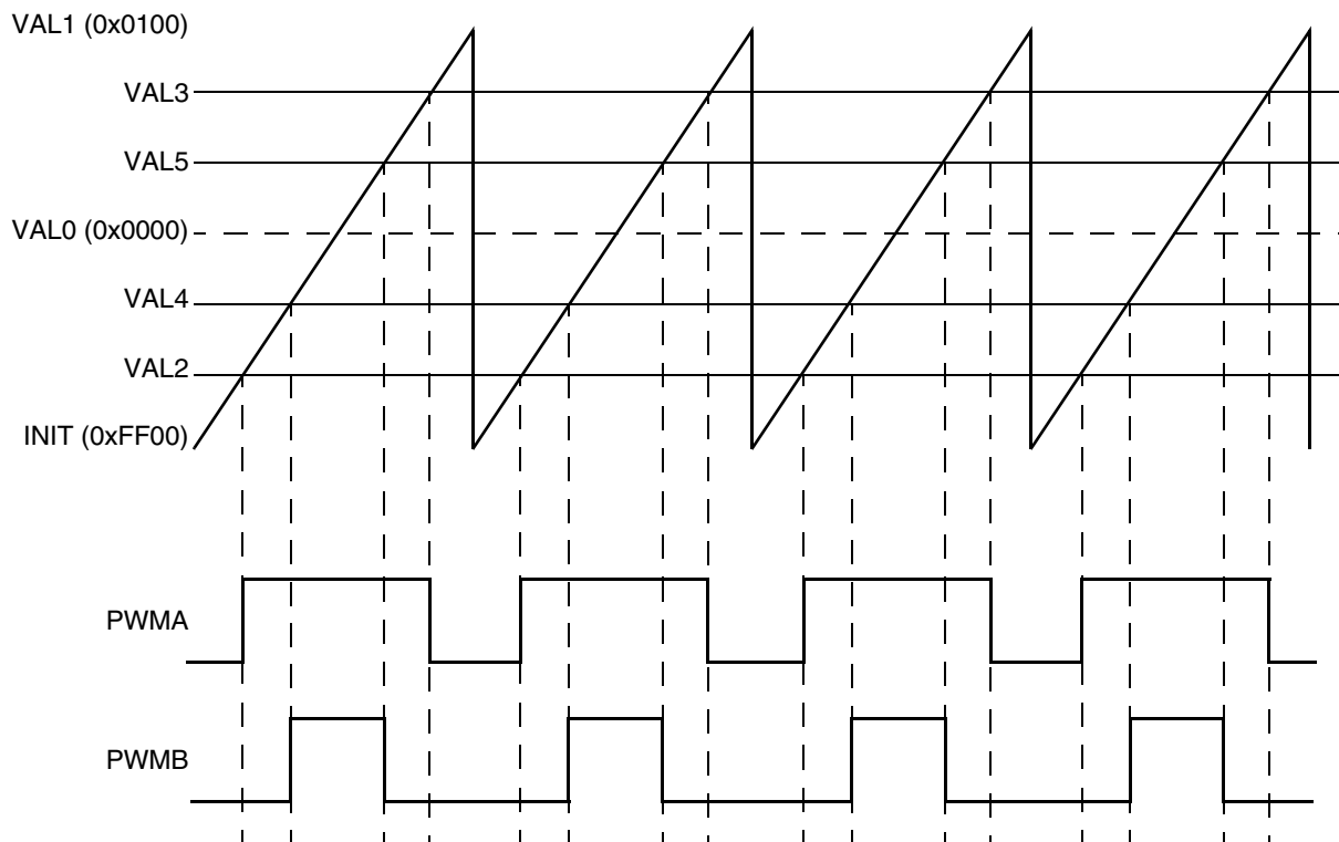
Figure 361. Center-aligned example
