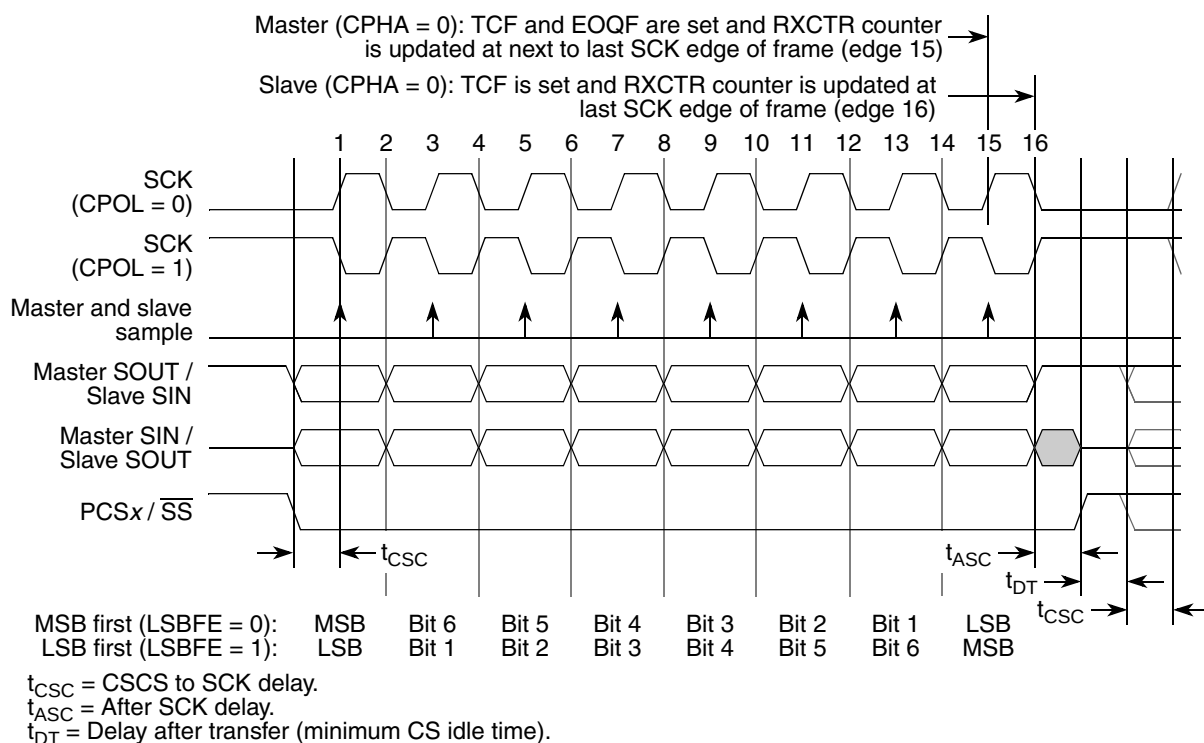
Figure 220. DSPI transfer timing diagram (MTFE = 0, CPHA = 0, FMSZ = 8)
