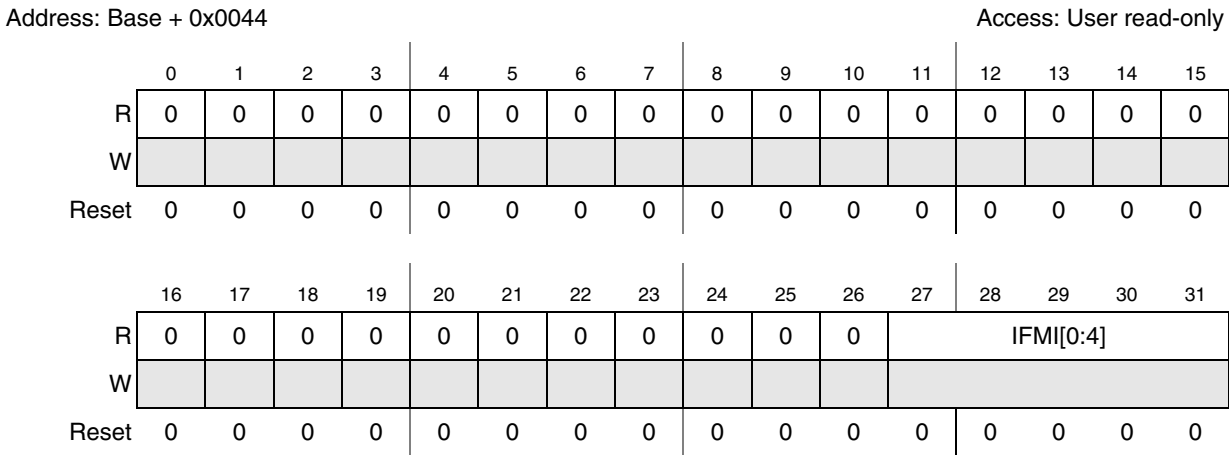
Figure 252. Identifier filter match index (IFMI)
