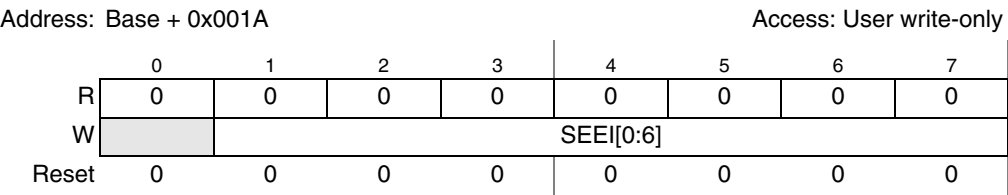
Figure 183. eDMA Set Enable Error Interrupt Register (EDMA_SEEIR)
