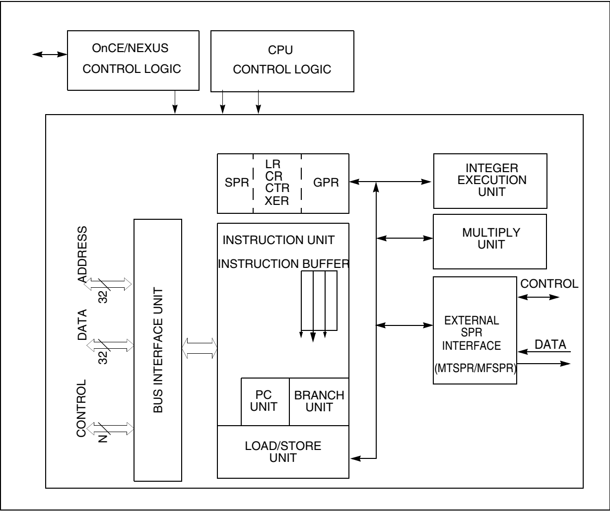
Figure 116. e200z0 block diagram
