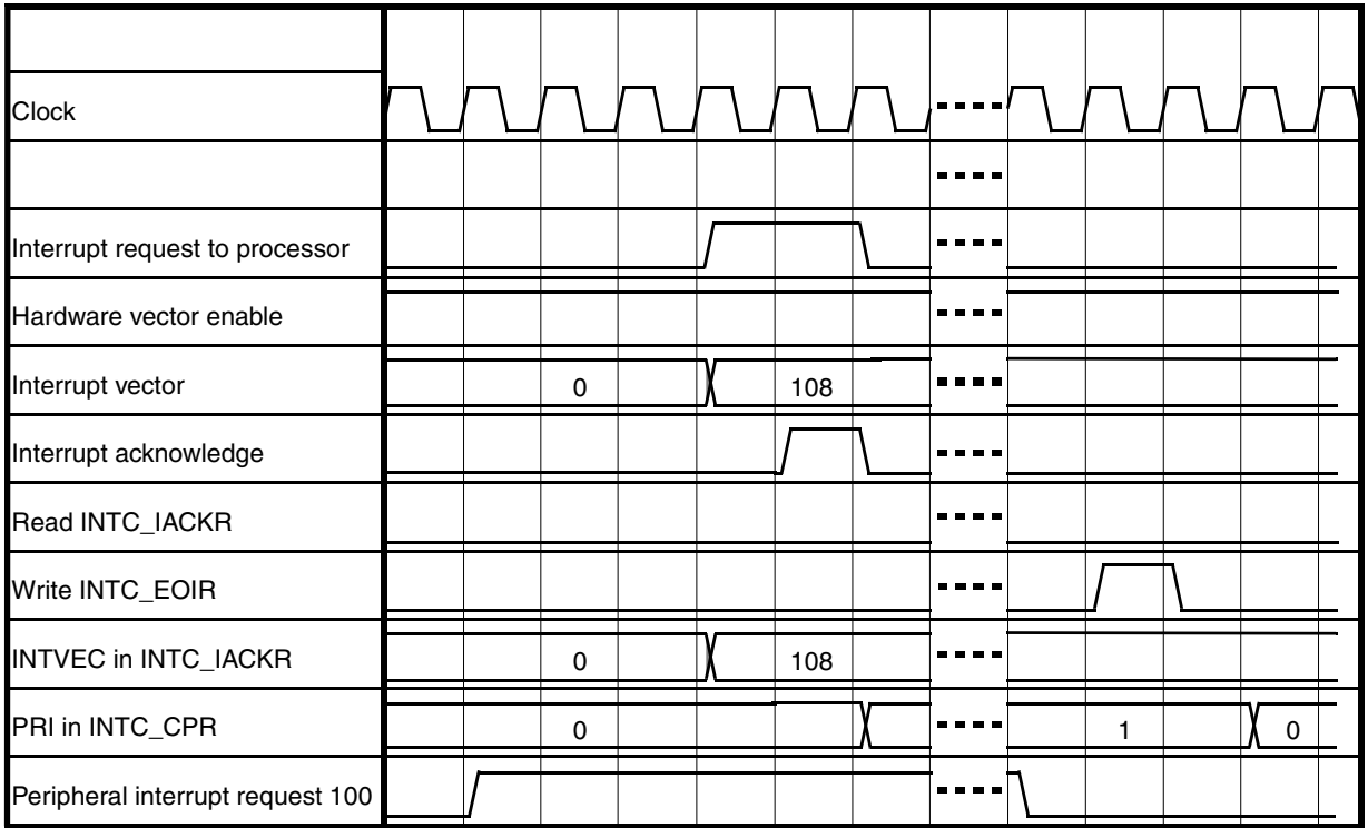
Figure 87. Hardware vector mode handshaking timing diagram
