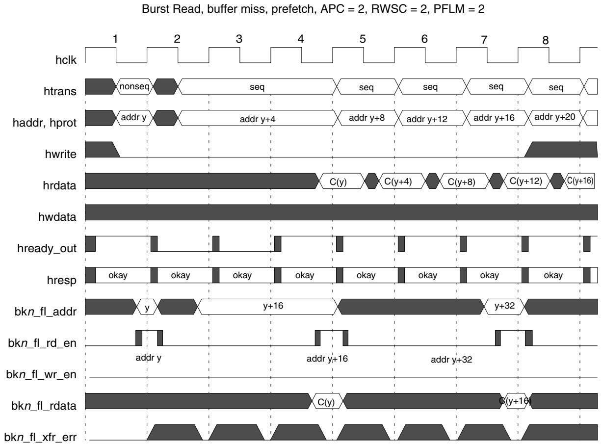
Figure 148. 3-cycle access, prefetch and buffering enabled
