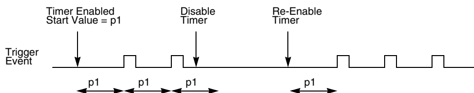
Figure 462. Stopping and starting a timer
