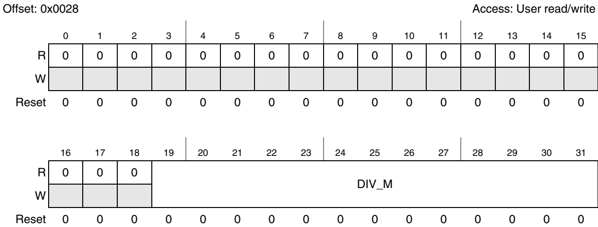
Figure 245. LIN integer baud rate register (LINIBRR)
