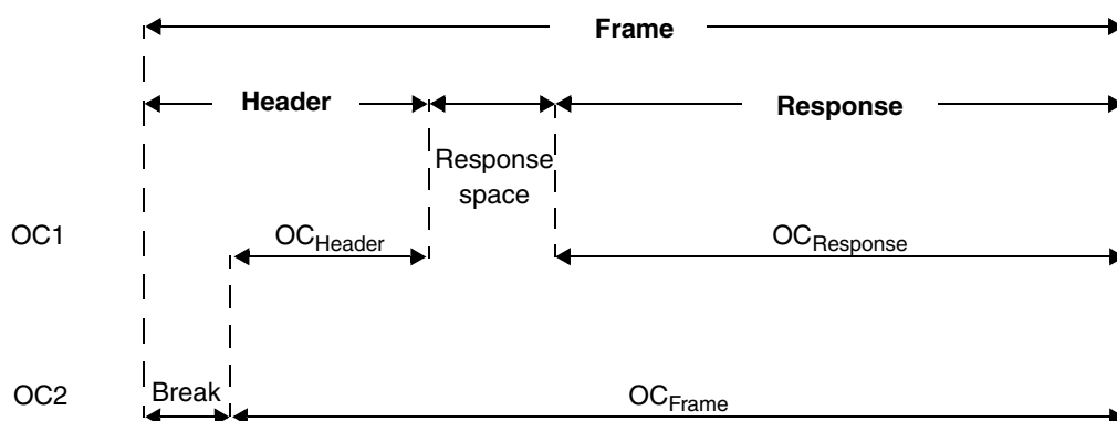
Figure 261. Header and response timeout
