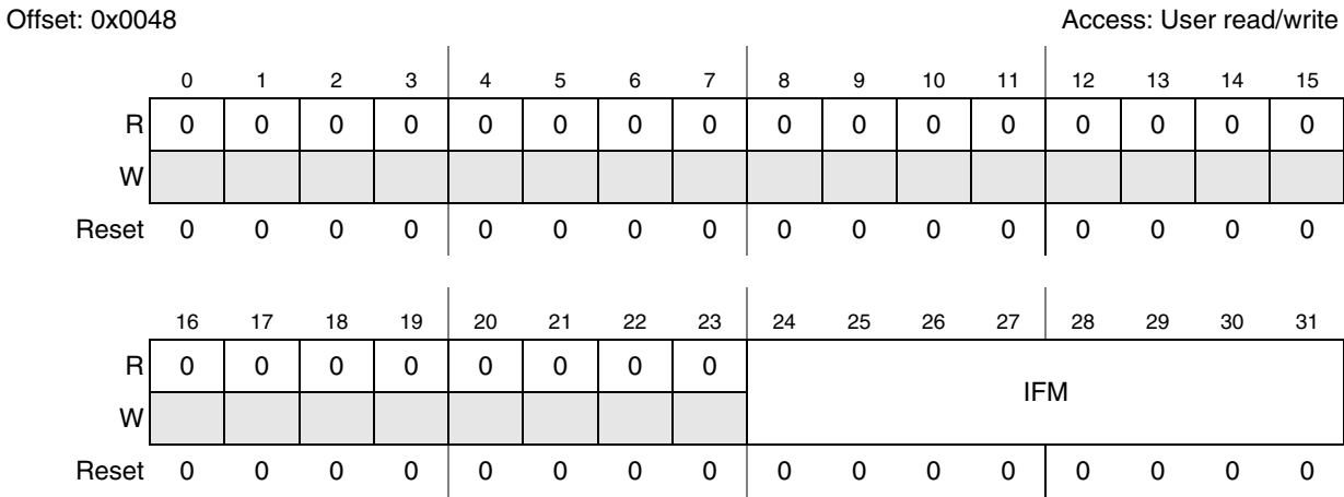
Figure 253. Identifier filter mode register (IFMR)
