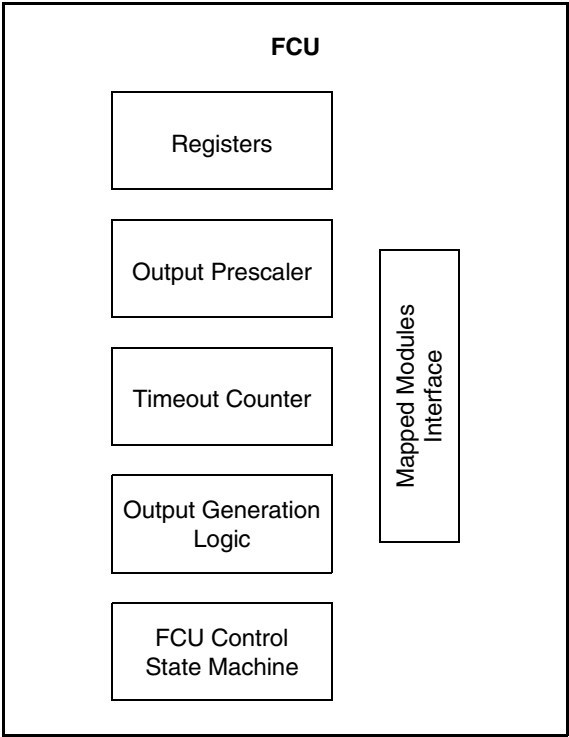
Figure 448. Functional block diagram
