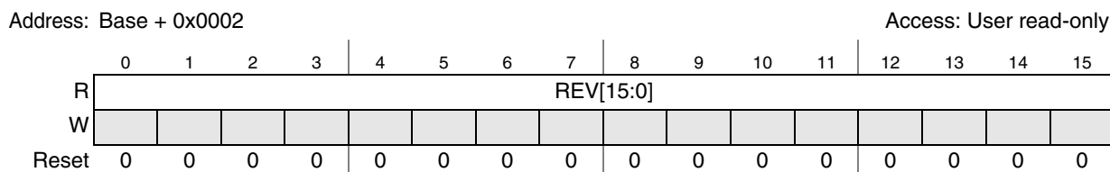
Figure 124. Revision (REV) register
