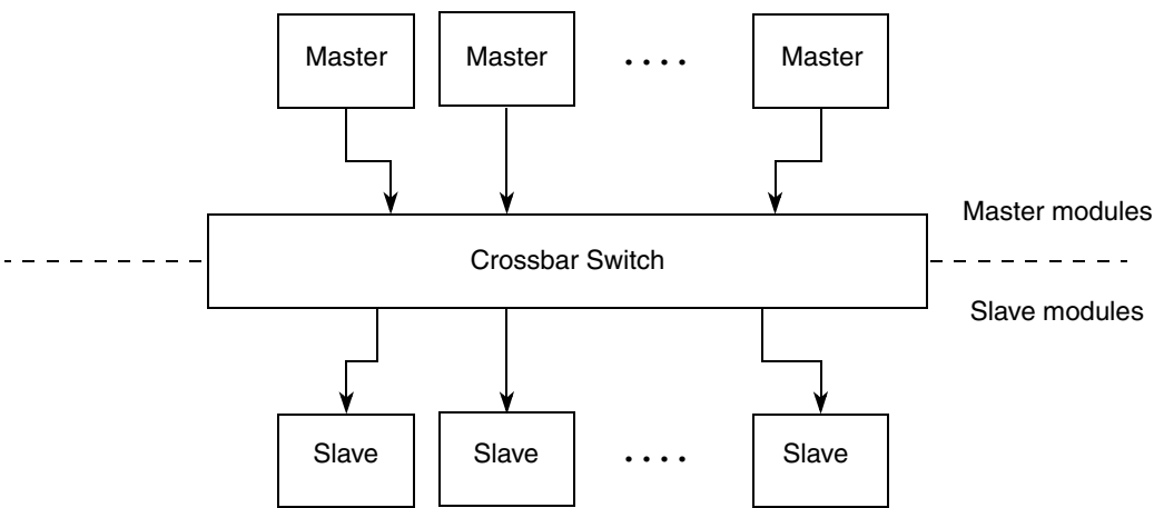
Figure 122. XBAR block diagram
