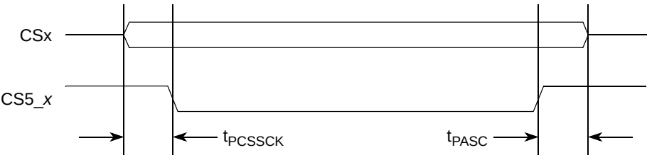
Figure 219. Peripheral Chip Select strobe timing
