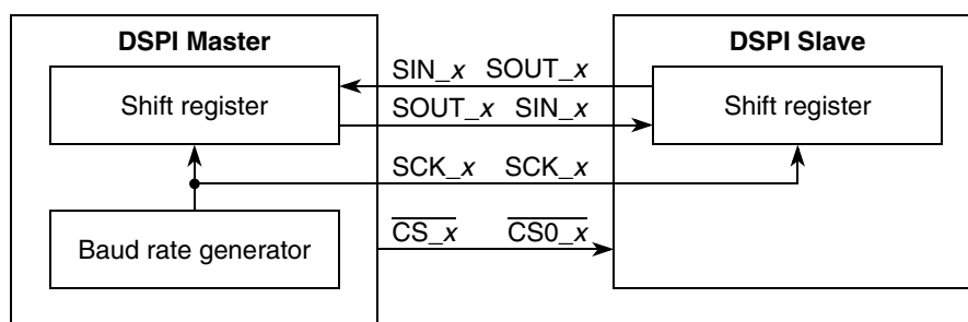
Figure 216. SPI serial protocol overview
