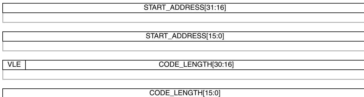
Figure 484. Start address, VLE bit and download size in bytes
