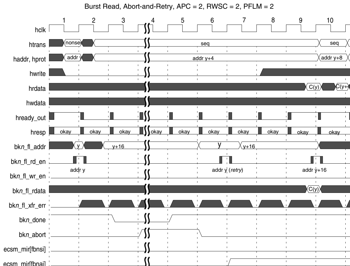
Figure 150. 3-cycle access, terminate-and-retry with BK_n\_RWWC = 10x
