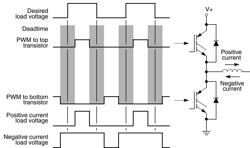
Figure 378. Deadtime distortion
