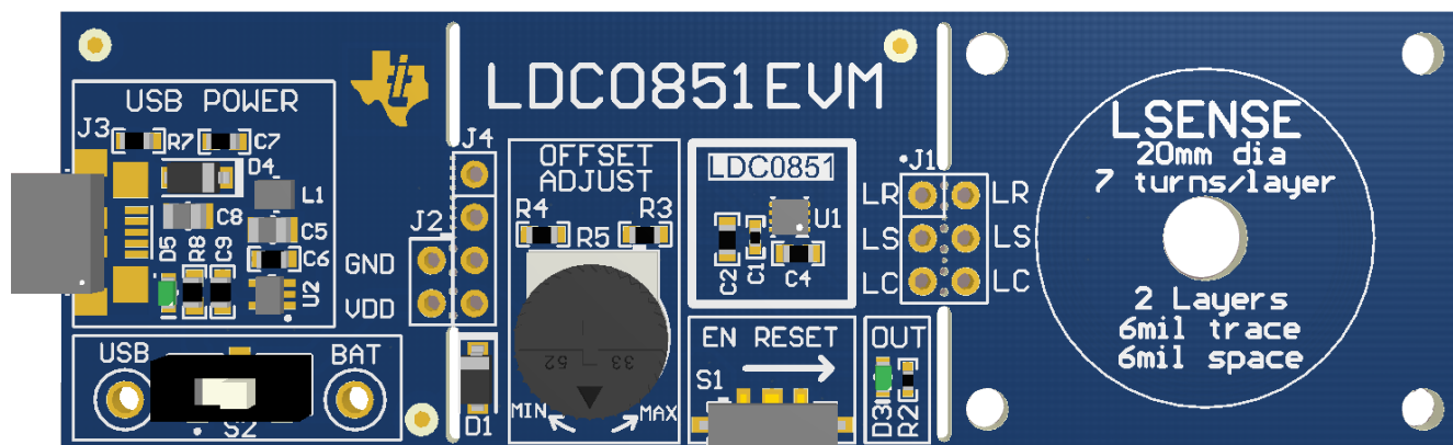
Figure 1. LDC0851EVM
