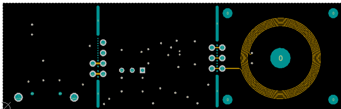
Figure 24. Mid-Layer 1 Routing
