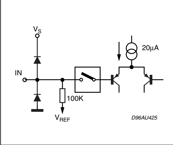
Figure 16. PINS: 1, 2, 3, 4, 5, 6, 7, 28
