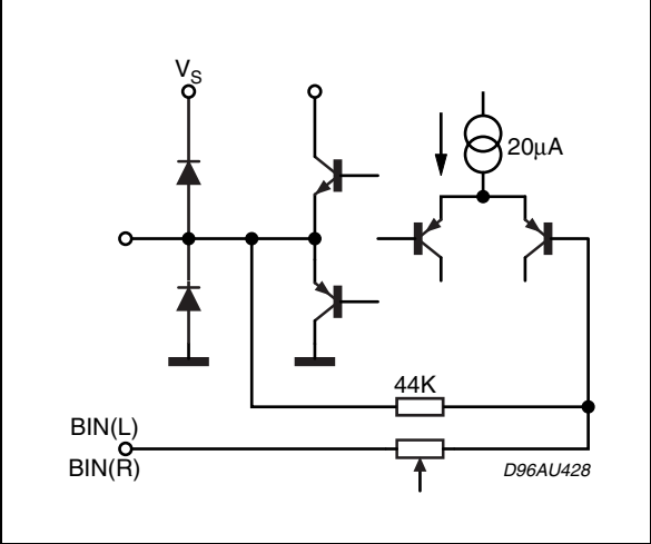
Figure 19. PINS: 12, 14
