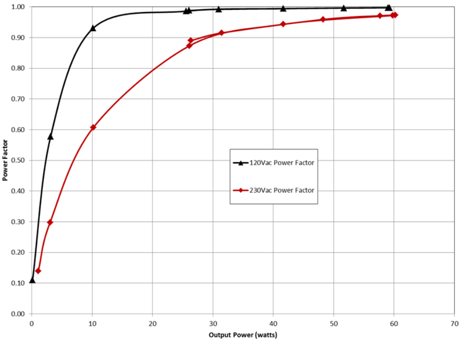
Figure 8. Power Factor over Load
