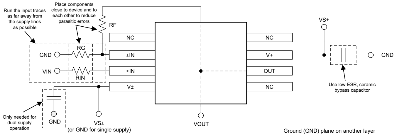
Figure 55. Operational Amplifier Board Layout for a Noninverting Configuration
