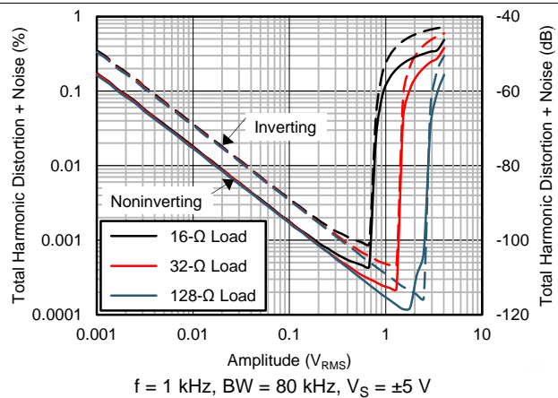
Figure 18. THD+N vs Amplitude
