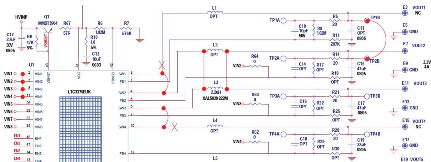
Figure 8. Combined 4A Output, Regulators 1, 2, 3 and 4
