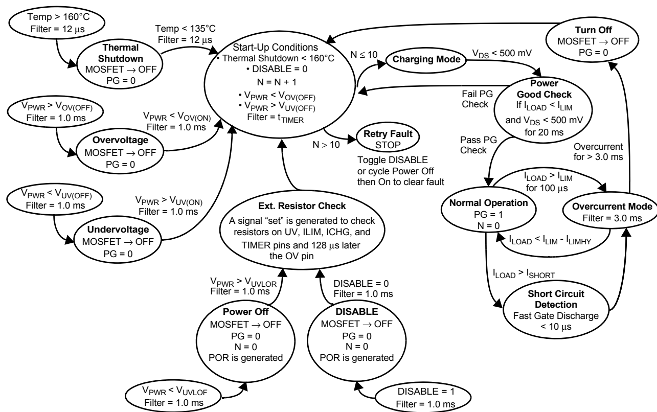
Figure 13. State Diagram
