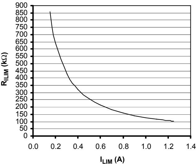
Figure 22. External Resistor ( R_{ILIM} ) Value Versus Current Limit Value ( I_{LIM} )
