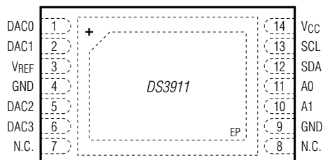
TDFN (3mm x 5mm)
