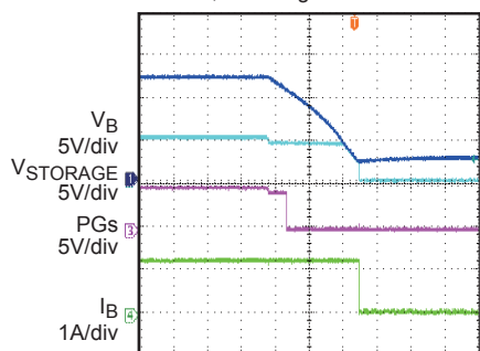
Release Time
