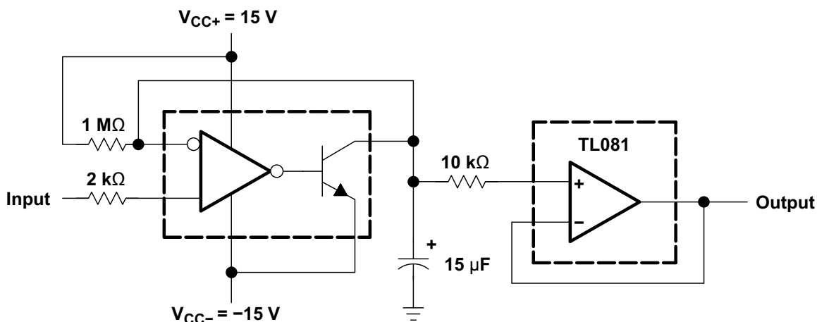
Figure 29. Negative-Peak Detector
