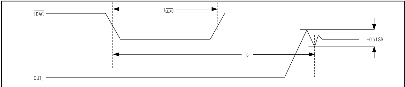
Figure 3. LDAC Timing
