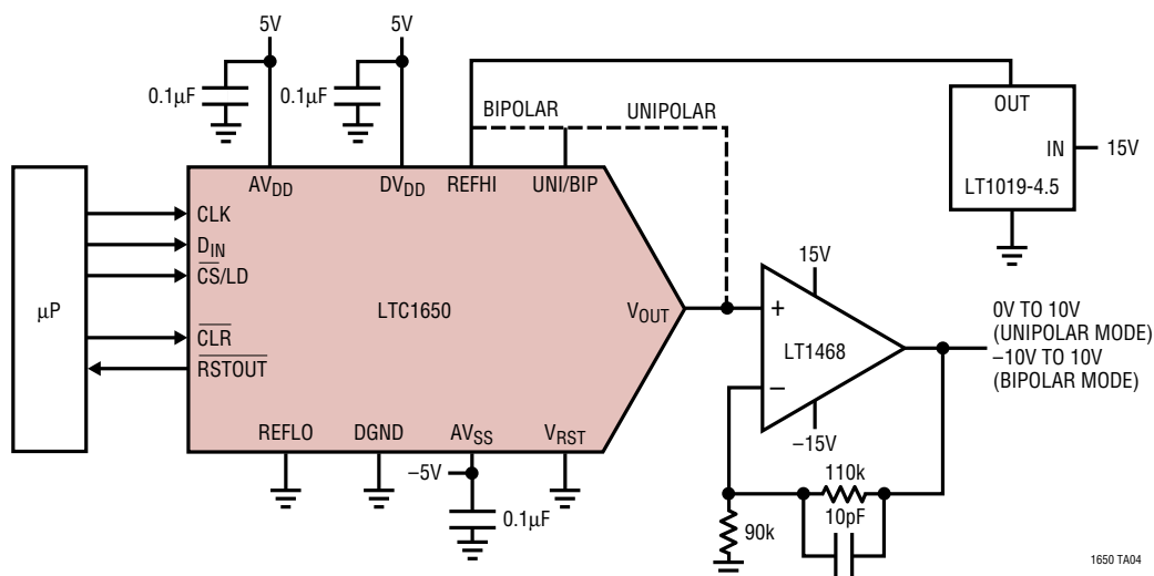
A \pm 10\text{V} Bipolar Output 16-Bit DAC
