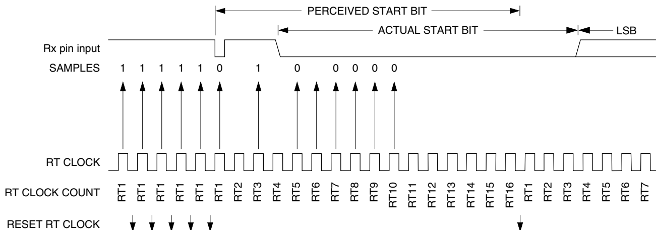
In the following figure, verification sample at RT3 is high. In this example C7816[ISO_7816E] = 0. The RT3 sample sets the noise flag. Although the perceived bit time is misaligned, the data samples RT8, RT9, and RT10 are within the bit time and data recovery is successful.
