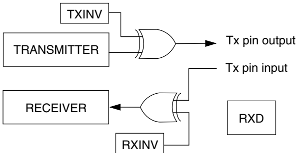
Figure 48-241. Single-wire operation (C1[LOOPS] = 1, C1[RSRC] = 1)
