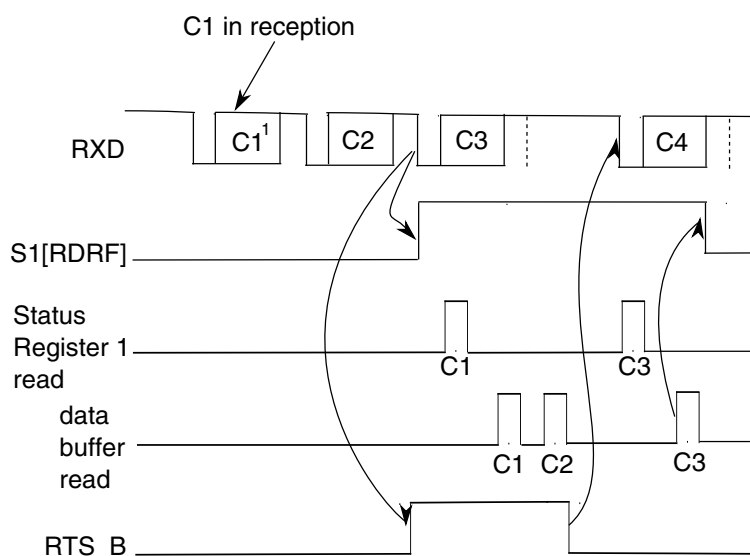
Figure 48-228. Receiver hardware flow control timing diagram
