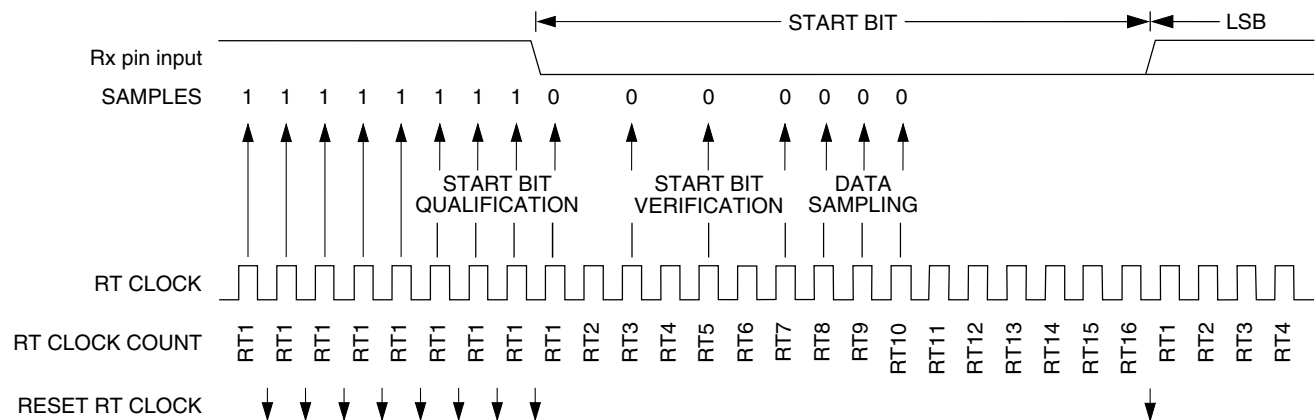
Figure 48-221. Receiver data sampling
