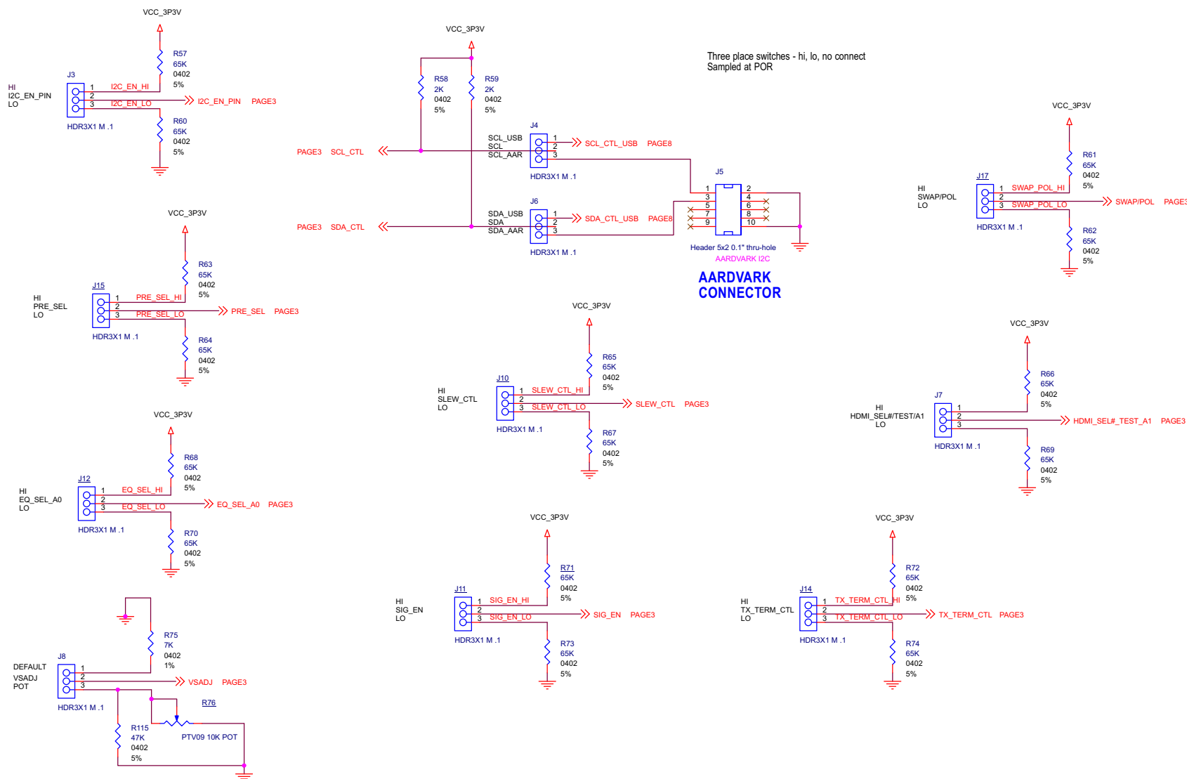
Figure 10. DP159RGZEVMS Select Options
