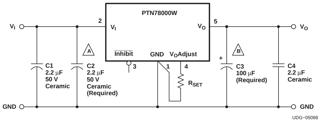
Figure 31. Adding High-Frequency Bypass Capacitors To The Input and Output
