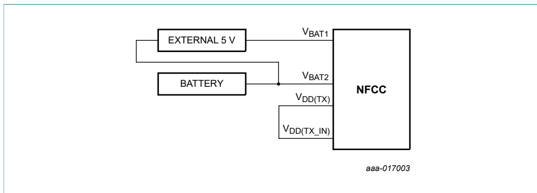
Fig 15. V_{BAT1} = 5\text{ V} , V_{BAT2} between 2.3 V and 5.5 V
