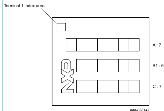
Figure 3. PN7150 package marking HVQFN40 (top view) 3 lines
