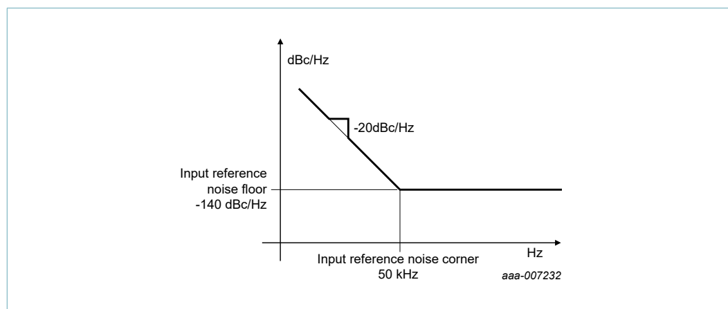
Fig 10. Input reference phase noise characteristics
