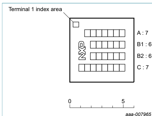
Figure 2. PN7150 package marking HVQFN40 (top view) 4 lines
