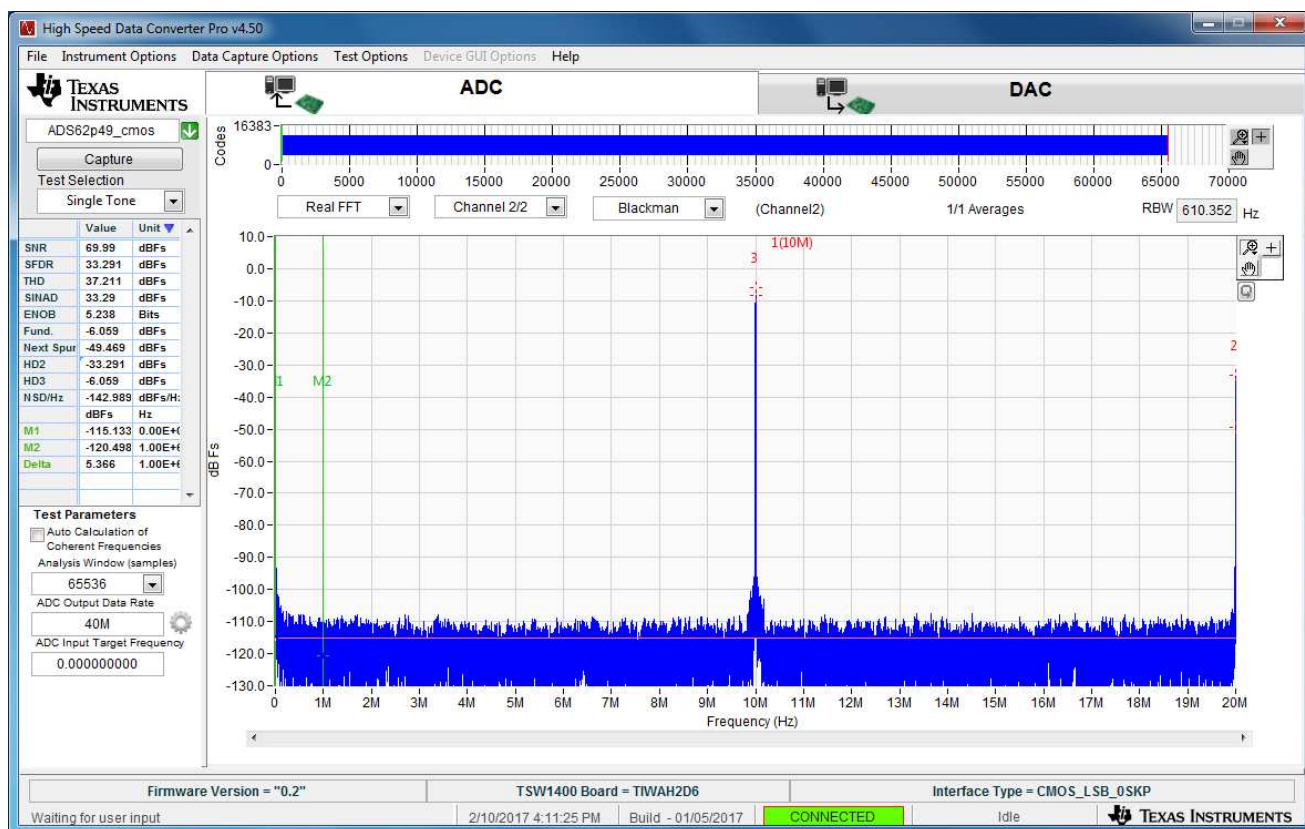
Figure 44. TSW1400EVM Captured Results from ADS62P49EVM
