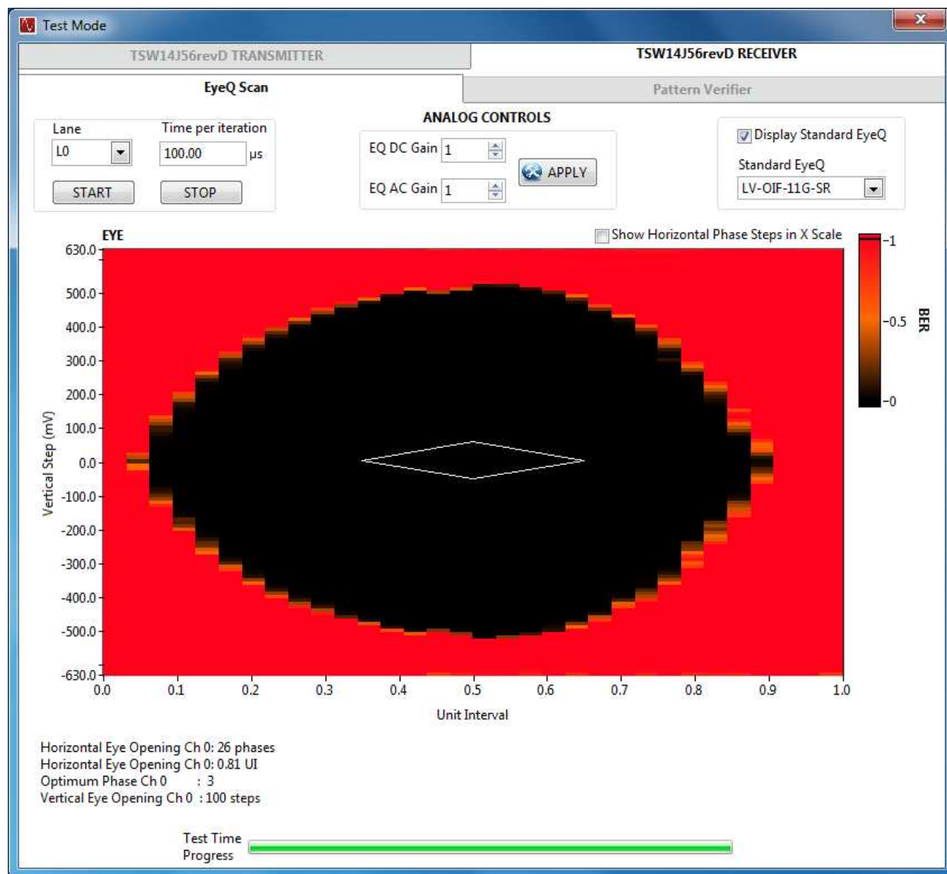
Figure 10. Example Eye Diagram Plot
