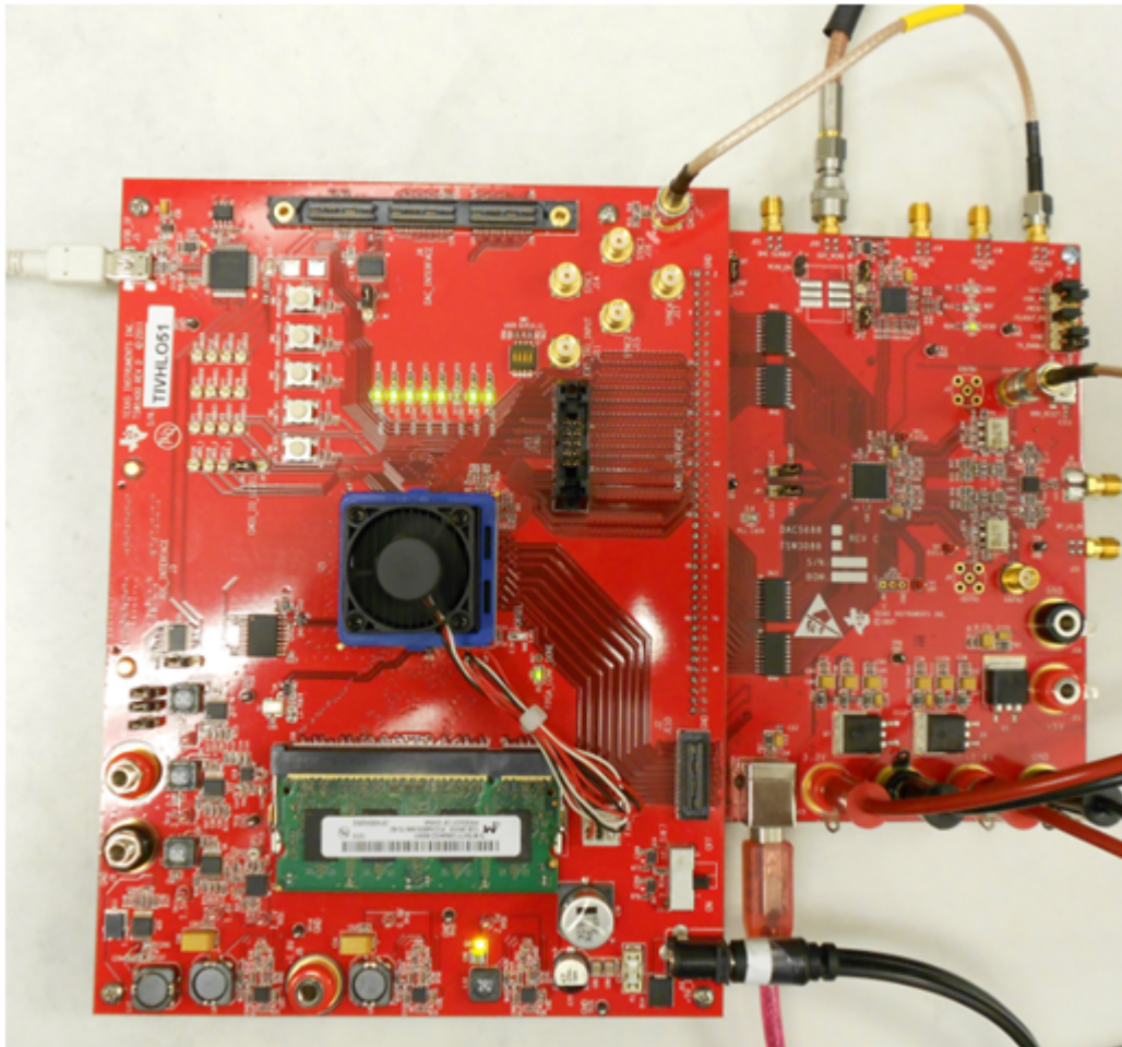
Figure 49. TSW1400EVM Interfacing to the CMOS Connectors of a DAC5688EVM
