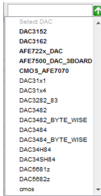
Figure 47. DAC Selection
