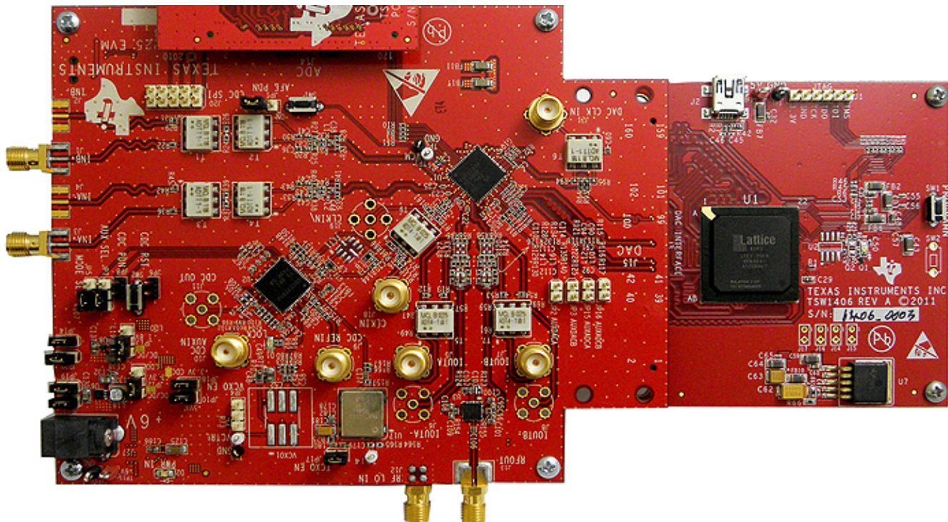
Figure 55. TSW1406 EVM Connected to the DAC input of the AFE7225 EVM
