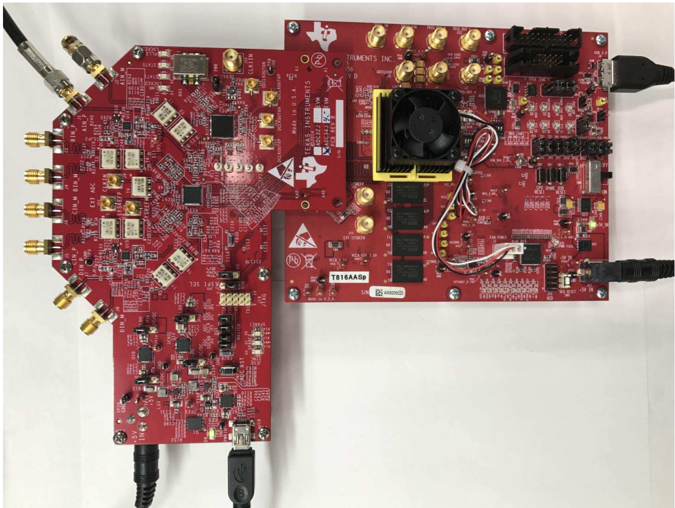
Figure 61. TSW14J56 EVM connected to an ADC34J45 EVM
