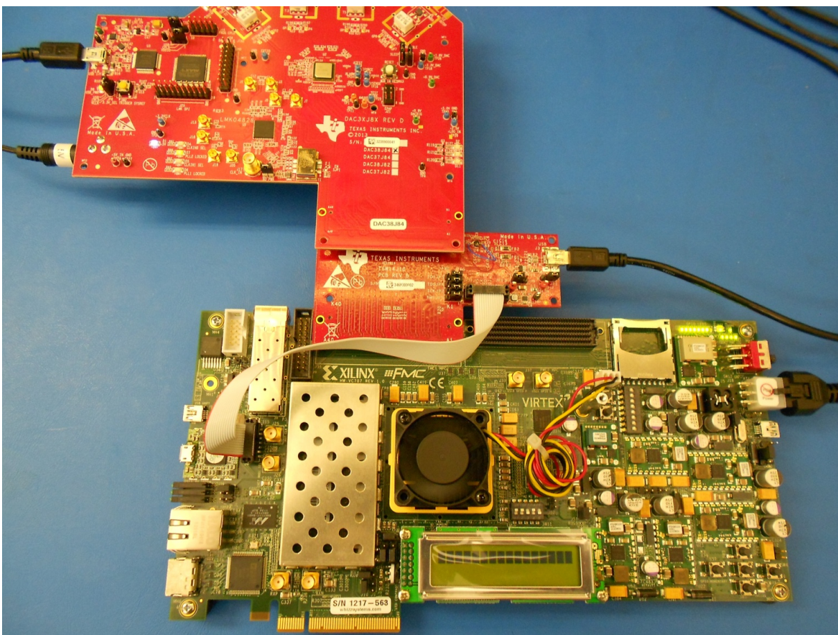
Figure 66. TSW14J10EVM, DAC38J84EVM, and Virtex VC707 Development Card
