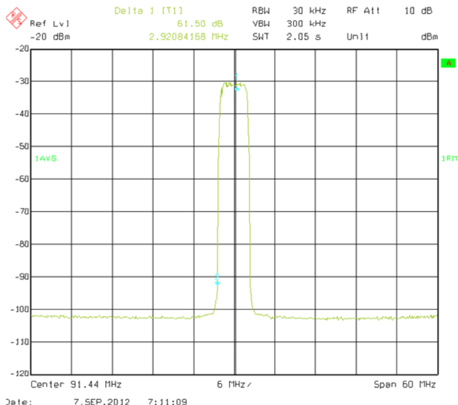
Figure 52. DAC5688 IF Output
