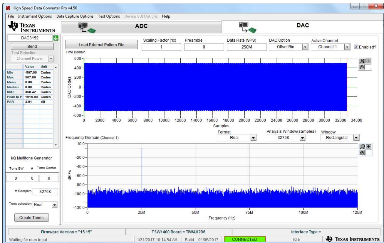
Figure 38. DAC Test Pattern Display
