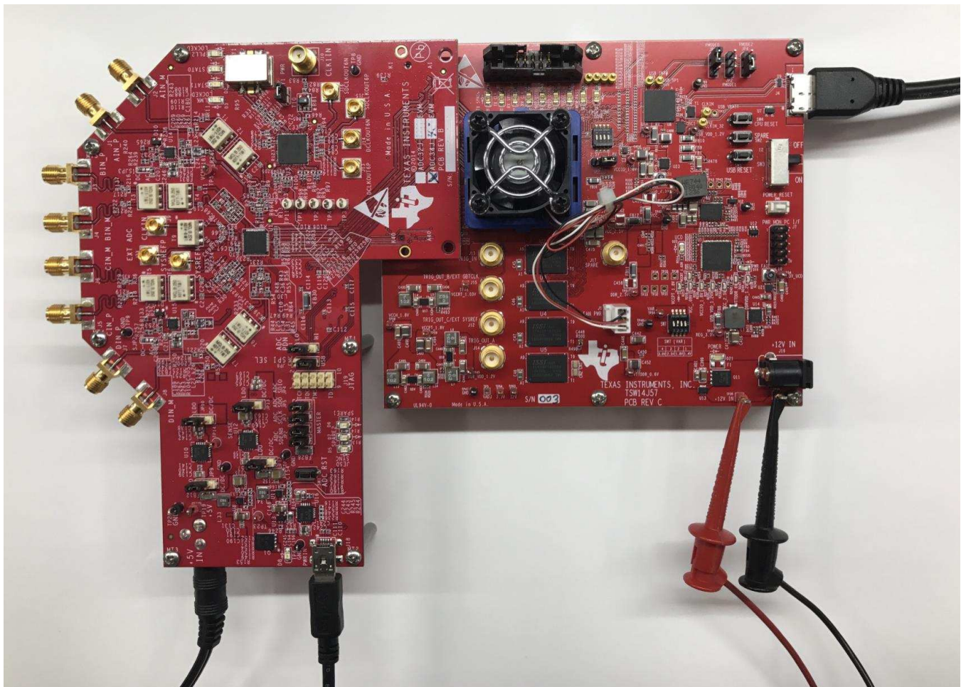
Figure 57. TSW14J57 EVM connected to an ADC34J45 EVM
