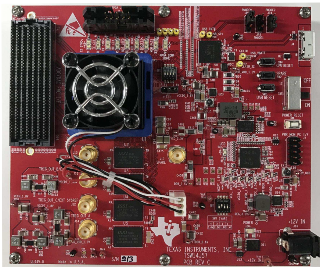
Figure 56. TSW14J57 EVM
