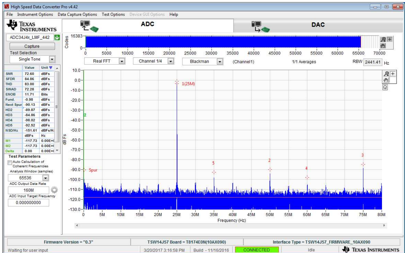
Figure 59. ADC34J45 Operating in 14-Bit Mode at 160 Msps with 25-MHz Input Signal
