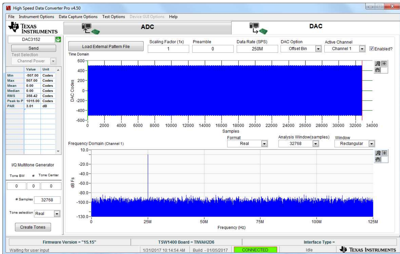
Figure 48. TSW1400 Output Data to DAC EVM
