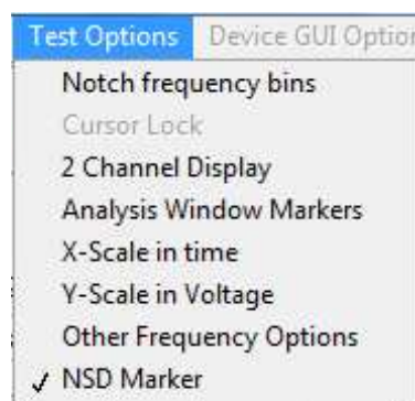
Figure 18. Test Options
