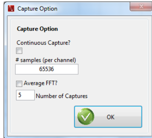
Figure 11. Capture Option
