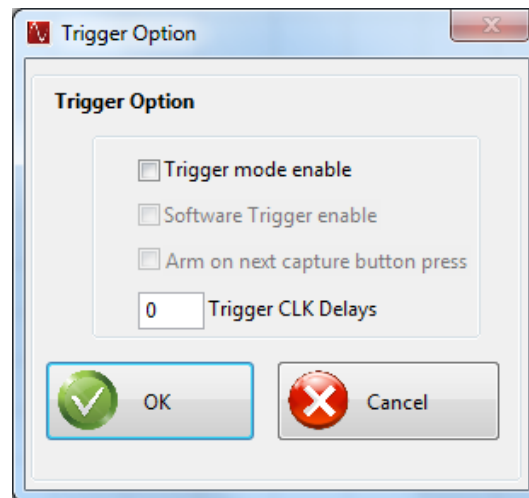
Figure 12. Trigger Option
