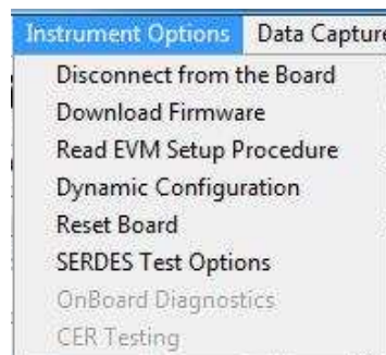
Figure 9. Instrument Options
