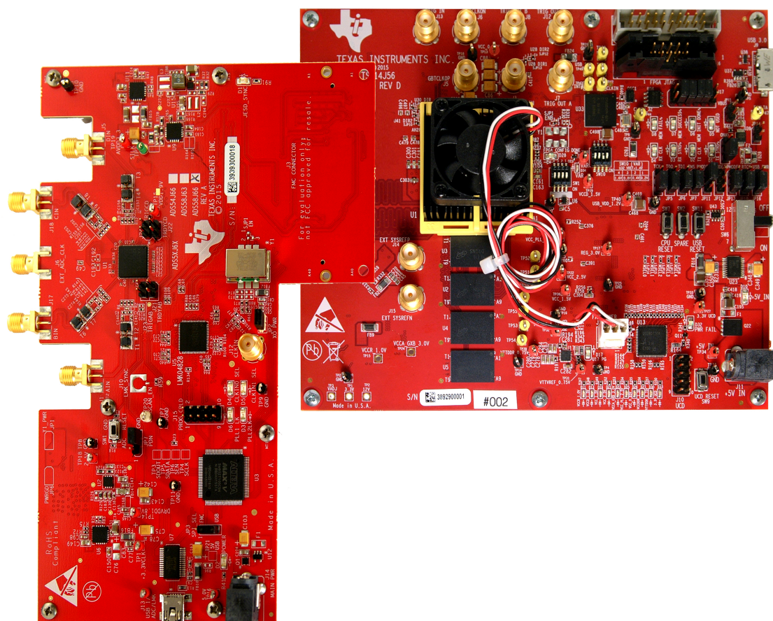
Figure 60. TSW14J56 EVM connected to an ADS58J63 EVM
