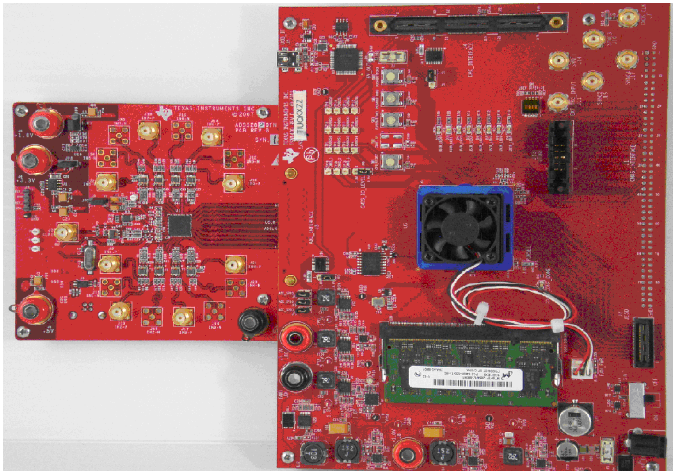
Figure 40. TSW1400EVM interfacing to an ADS5281 EVM
