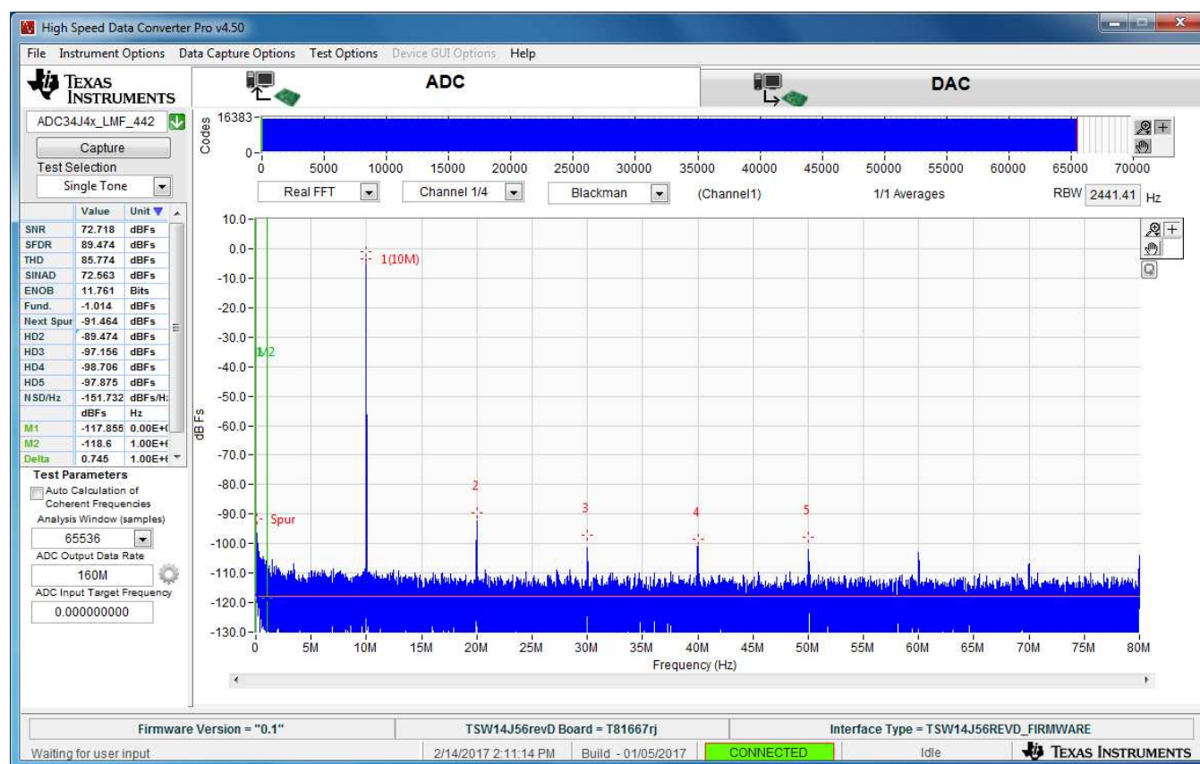
Figure 63. ADC34J45 Operating in 14-Bit Mode at 160 Msps with 10-MHz Input Signal
