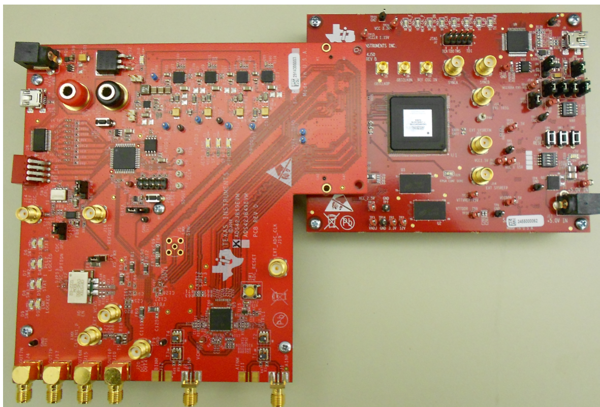
Figure 64. TSW14J50 EVM Connected to an ADS42JB69 EVM
