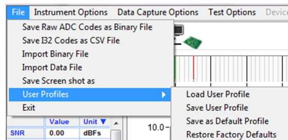
Figure 8. User Profiles
