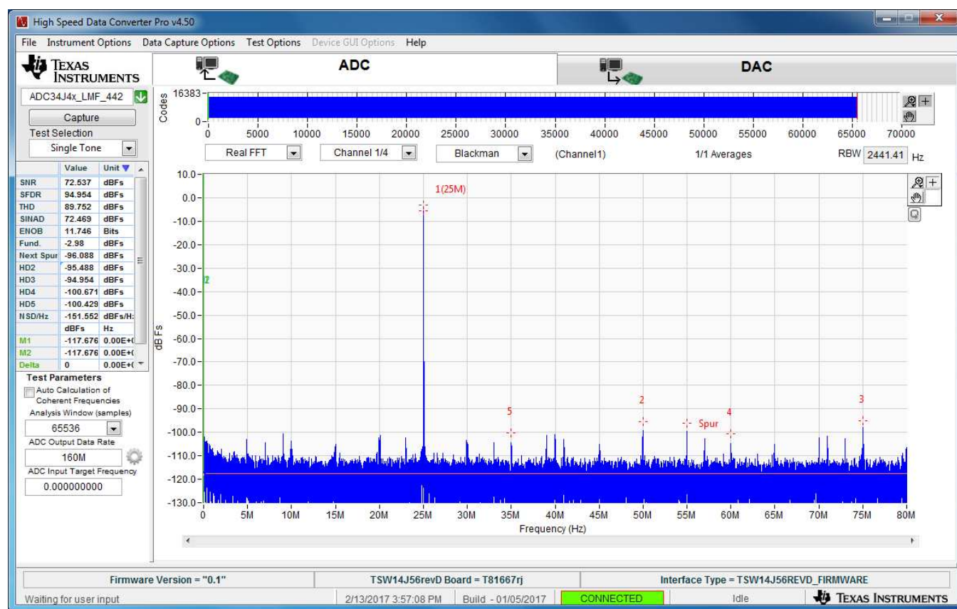
Figure 28. Single Tone FFT Display
