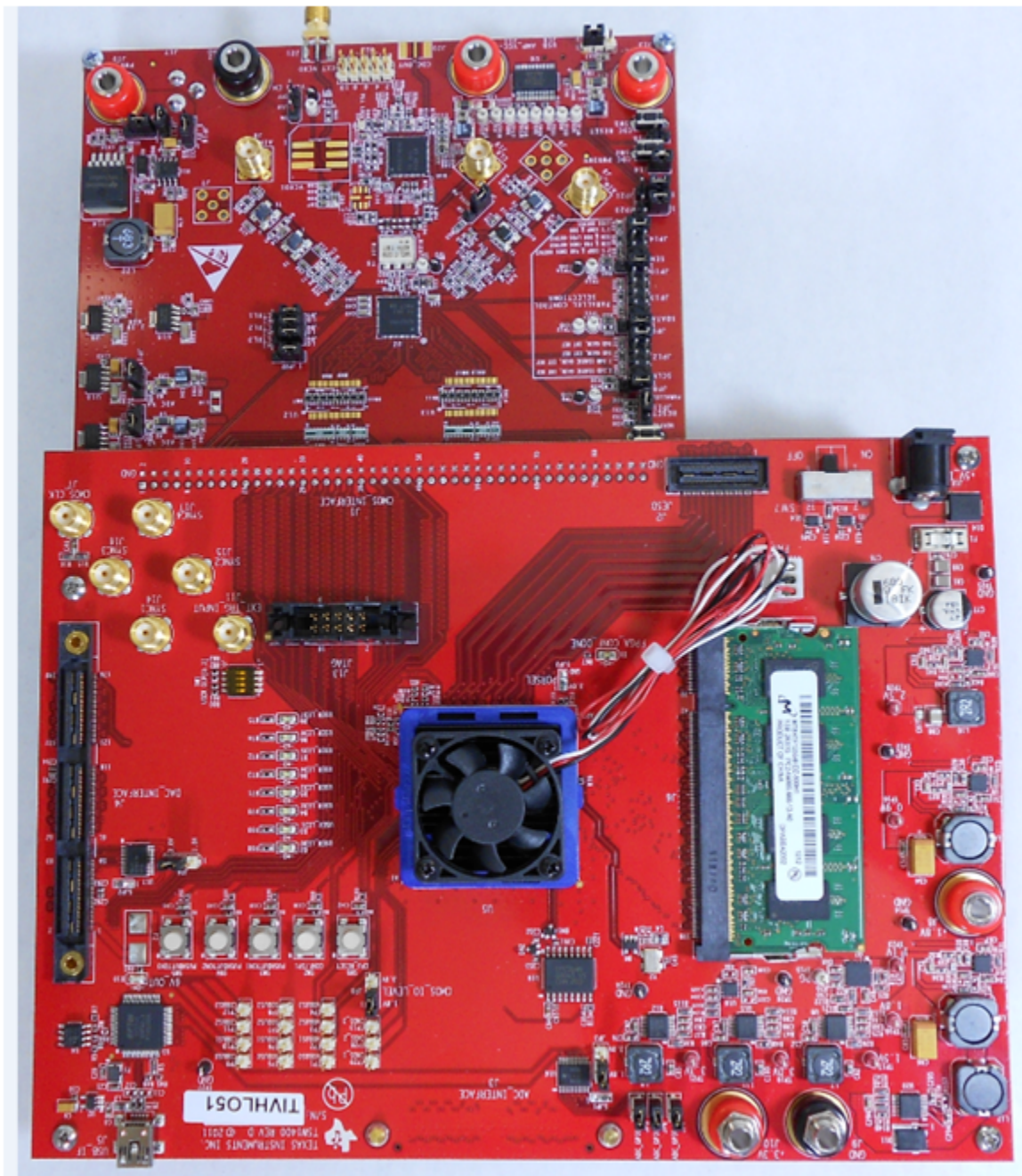
Figure 43. TSW1400EVM interfacing to the CMOS connectors of an ADS62P49EVM
