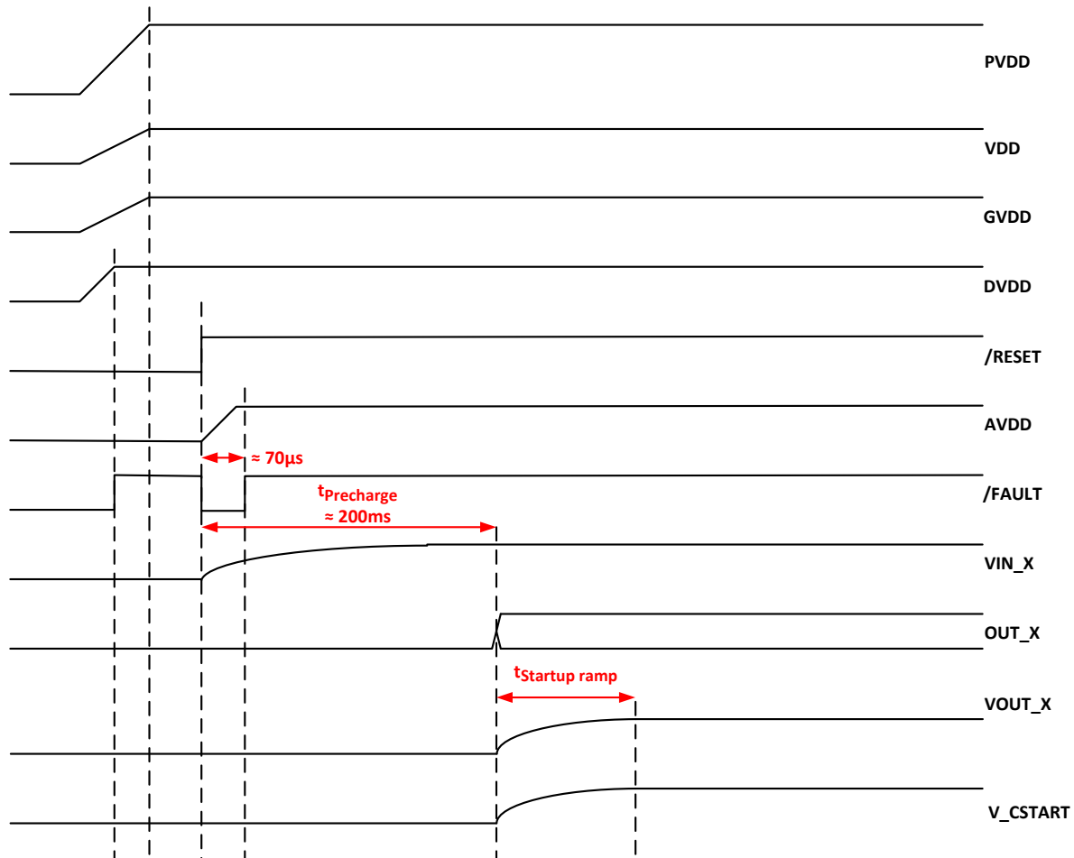
Figure 27. Startup Timing
