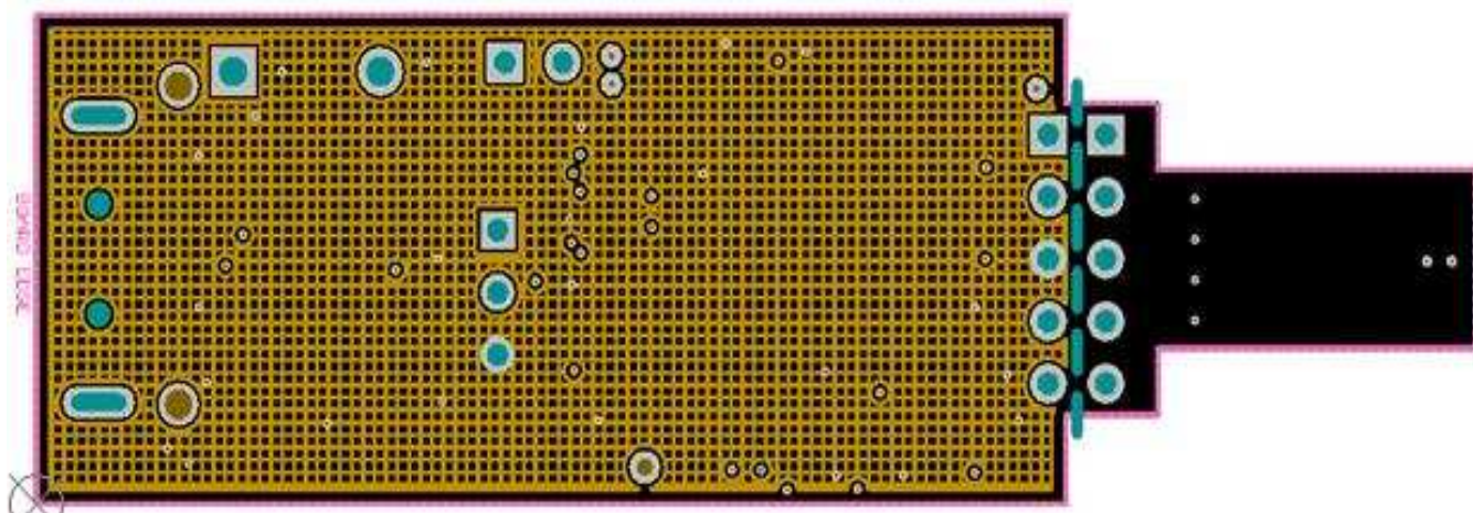
Figure 24. Ground Layer Routing
