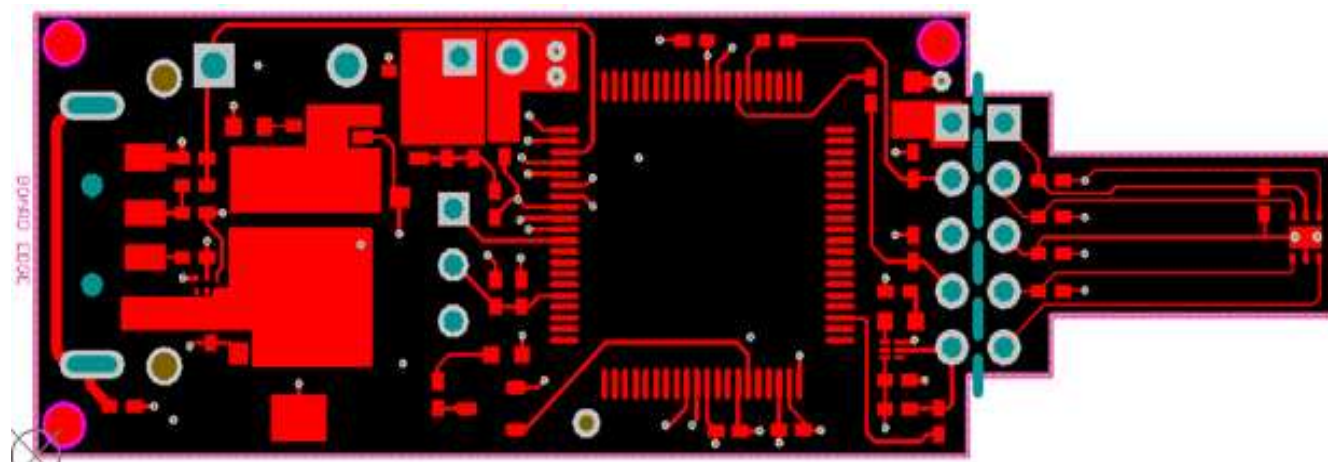
Figure 22. Top Layer Routing
