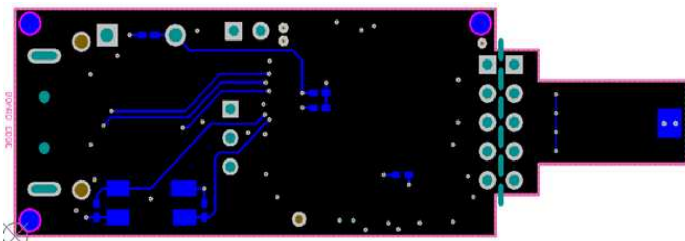
Figure 25. Bottom Layer Routing
