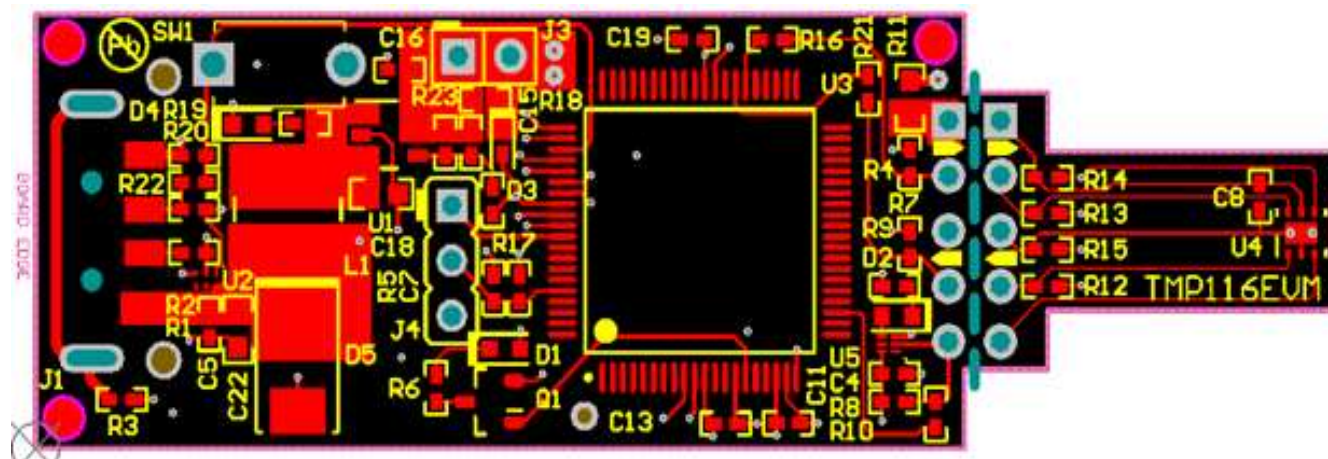
Figure 21. Top Assembly Layer
