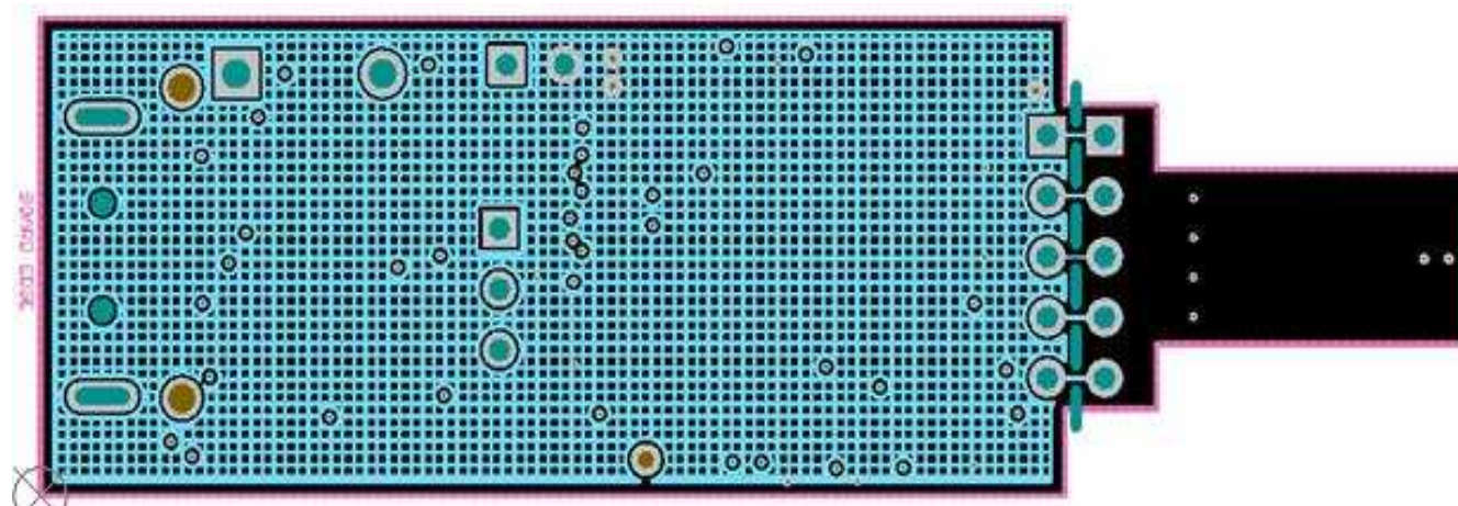
Figure 23. Power Layer Routing
