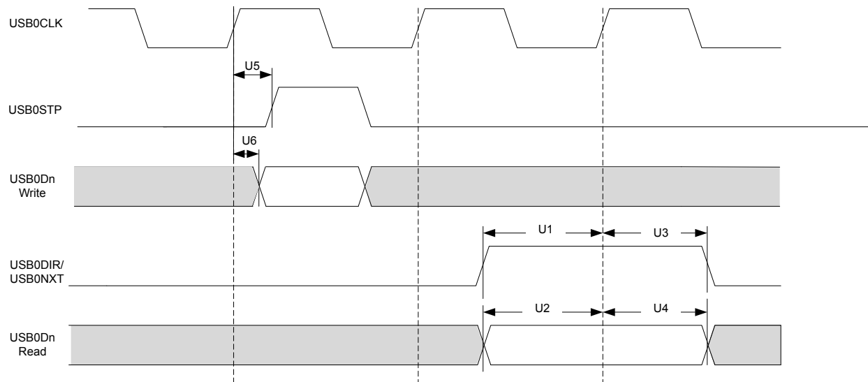
Figure 26-34. ULPI Interface Timing Diagram
