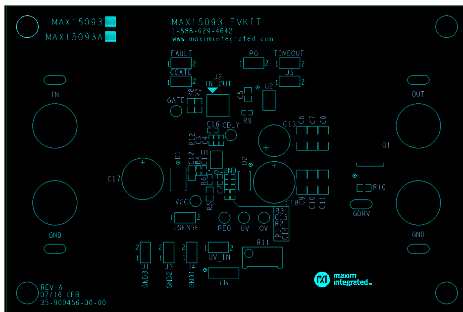
Figure 1. Component Placement Guide (Component Side)
