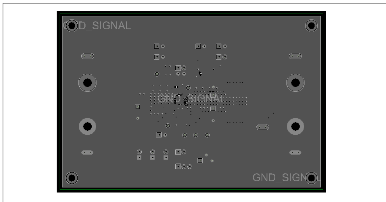
Figure 3. PCB Layout (Layer 2 (GND))
