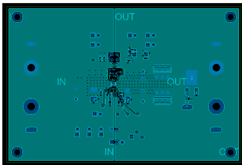
Figure 2. PCB Layout (Component Side)
