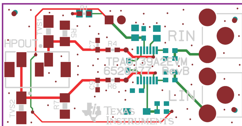
Figure 5. Bottom Silkscreen
