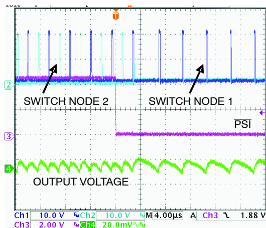
Figure 20. \overline{PSI} Transition
