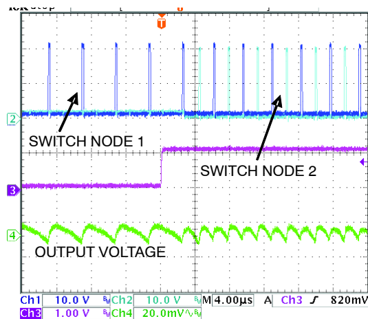
Figure 21. \overline{PSI} Transition
