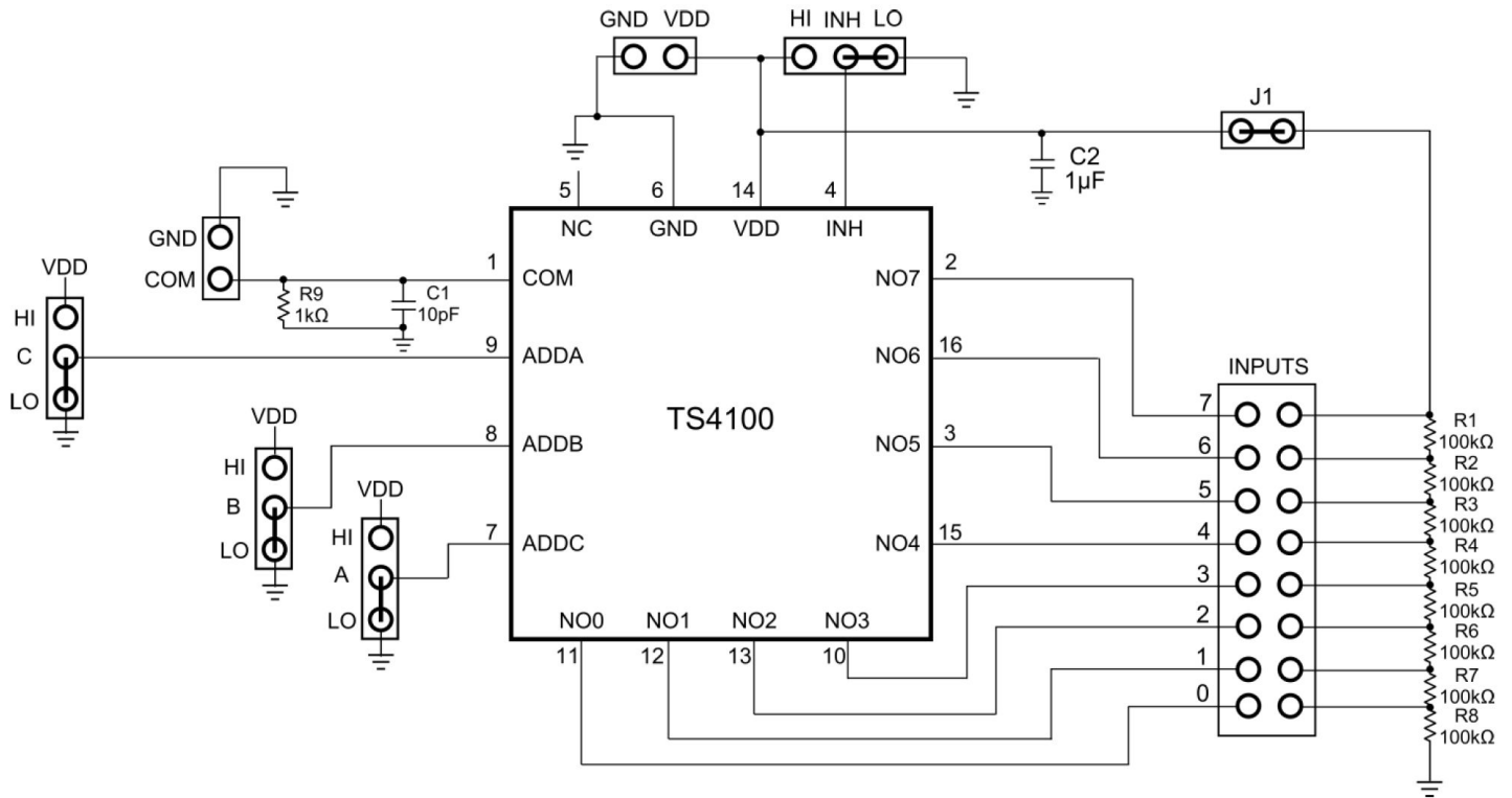
Figure 2.1. TS4100DB Schematic
