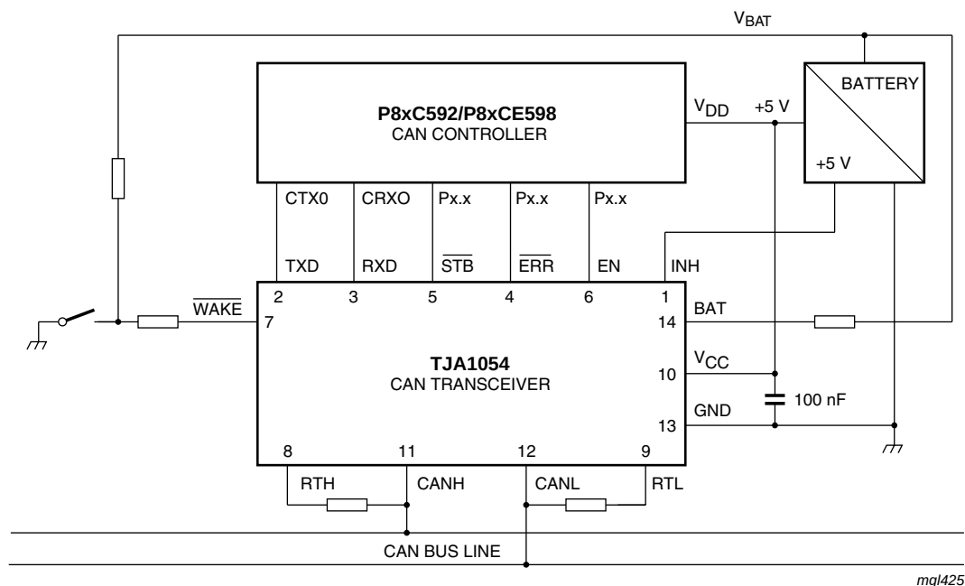
Fig 7. Application diagram
