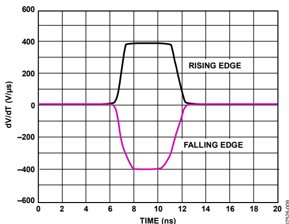
Figure 9. ADV3202 Slew Rate
