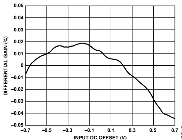
Figure 10. ADV3202 Differential Gain, Carrier Frequency = 3.58 MHz, Subcarrier Amplitude = 300 mV p-p
