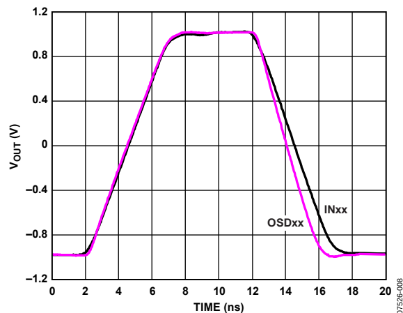
Figure 8. ADV3202 Large Signal Pulse Response, 2 V p-p
