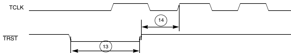
Figure 26. TRST Timing
