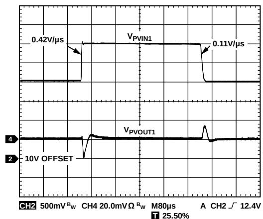
Figure 29. Buck Line Transient, V_{PVIN1} = 12V to 13V , V_{PVOUT1} = 1.2V , I_{LOAD1} = 1A , f_{SW} = 0.6MHz , L = 2.2μH , R_C = 3.48kΩ , C_C = 2nF , C_{CP} = 22pF , C_{PVOUT1} = 44μF
