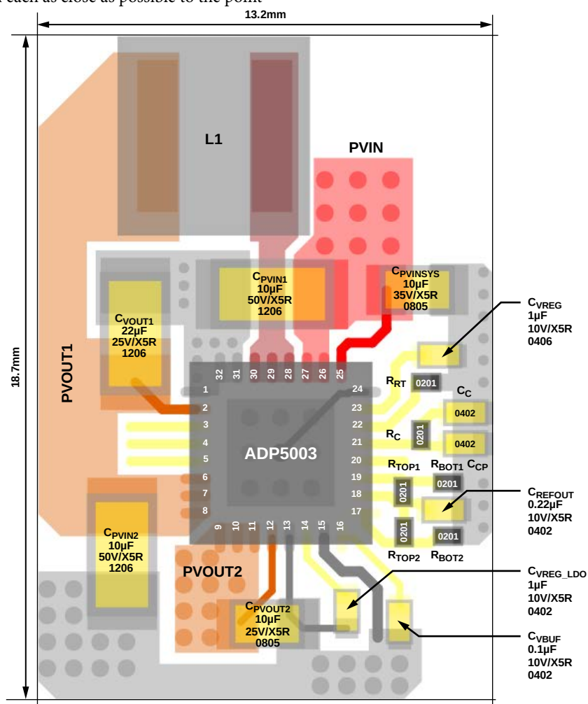
Figure 53. Example Outline Layout
