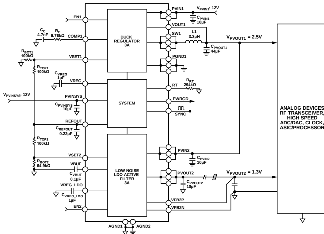
Figure 50. Independent Configuration (Dual Output)
