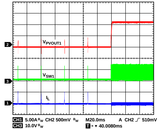
Figure 30. Exiting Hiccup Mode
