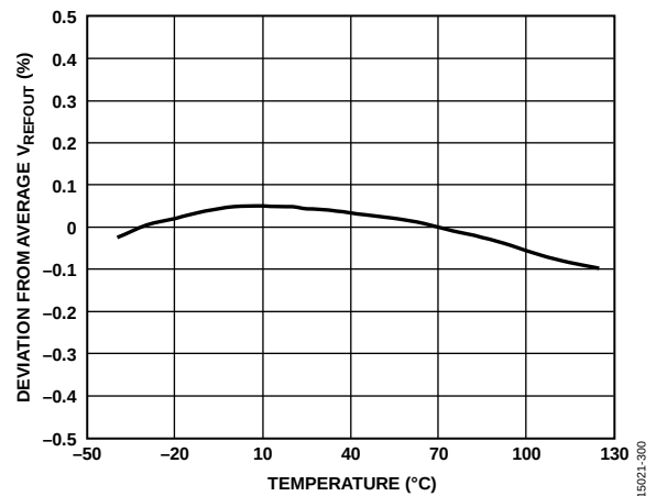
Figure 20. REFOUT Voltage ( V_{REFOUT} ) vs. Temperature
