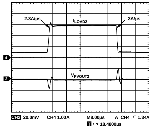
Figure 36. LDO Load Transient, V_{PVIN2} = 3.6\text{ V} , V_{PVOUT2} = 3.3\text{ V} , I_{LOAD2} = 0.5\text{ A to }3\text{ A}
