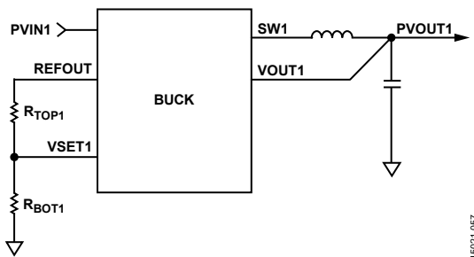
Figure 44. Buck Regulator Adjustable Output Voltage
