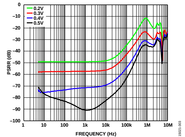
Figure 13. LDO PSRR vs. Frequency, V_{PVOUT2} = 3.3\text{ V} , I_{LOAD2} = 1\text{ A} at Various LDO Headroom Voltages
