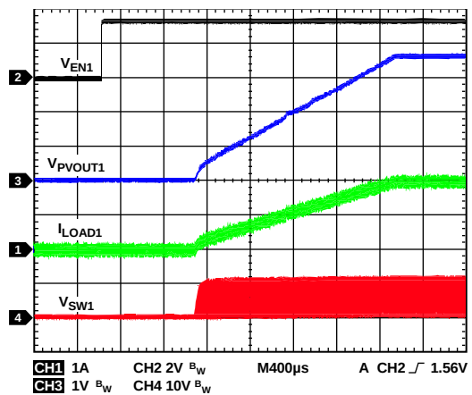
Figure 28. Buck Startup, V_{PVOUT1} = 3.3V , I_{LOAD1} = 3A ( V_{EN1} is the EN1 voltage.)
