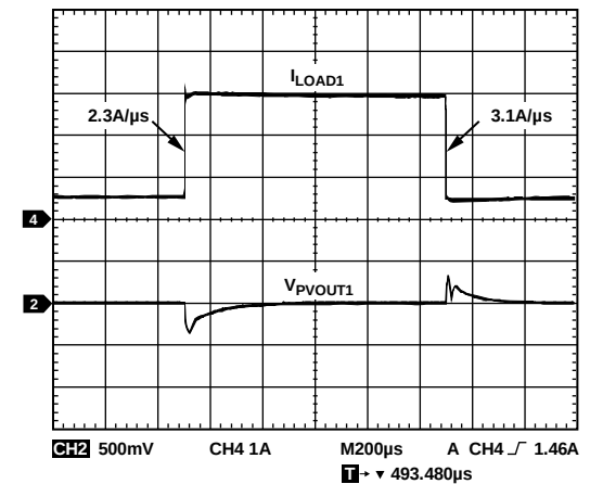
Figure 32. Buck Load Transient, V_{PVIN1} = 12V , V_{PVOUT1} = 1.2V , I_{LOAD1} = 0.5A to 3A , f_{SW} = 0.6MHz , L = 2.2μH , R_C = 3.48kΩ , C_C = 2nF , C_{CP} = 22pF , C_{PVOUT1} = 44μF
