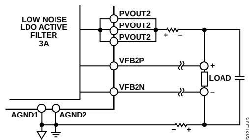
Figure 42. Differential Remote Sensing
