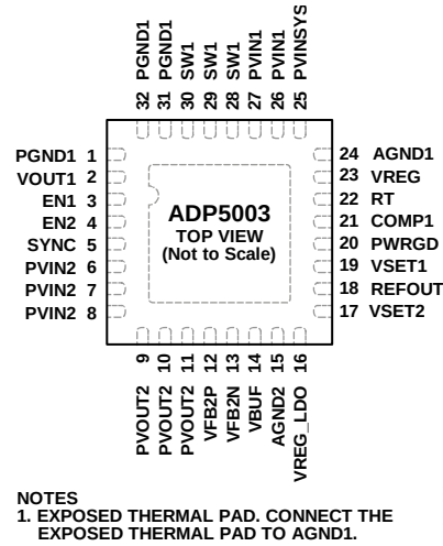
Figure 2. Pin Configuration
