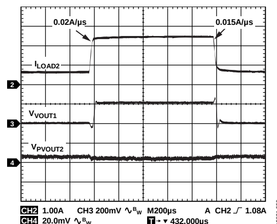
Figure 47. 0.6 A to 2.4 A Load Transient for 2.5 V Output, f_{SW} = 0.6 MHz, L = 3.3 \mu H, R_C = 9.76 k \Omega , C_C = 4.7 nF, C_{CP} = 4.7 pF, C_{PVOUT1} = 44 \mu F
