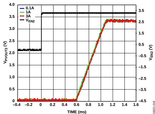
Figure 41. LDO Startup
