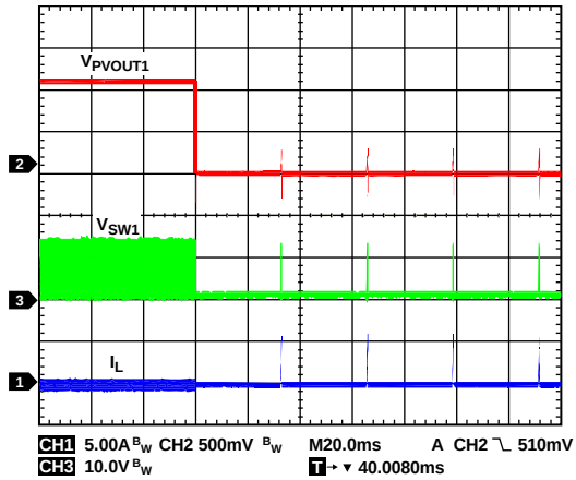
Figure 27. Entering Hiccup Mode ( V_{SW1} is the Voltage of the SW1 Pin, and I_L is Inductor Current)
