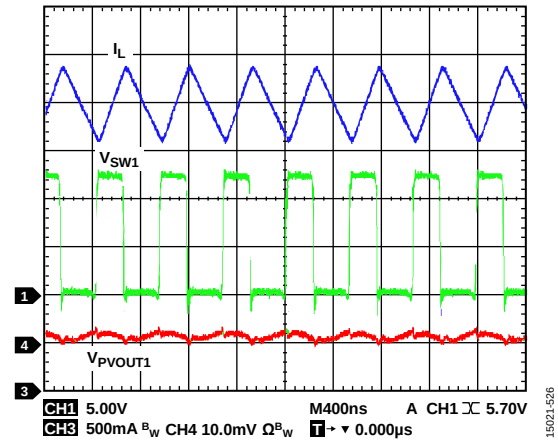
Figure 26. SW1 Waveform, V_{PVOUT1} = 5\text{ V} , I_{LOAD1} = 3\text{ A} , f_{SW} = 2\text{ MHz} , L = 2.2\text{ }\mu\text{H} , R_C = 2.7\text{ k}\Omega , C_C = 22\text{ nF} , C_{CP} = 22\text{ pF} , C_{PVOUT1} = 22\text{ }\mu\text{F}
