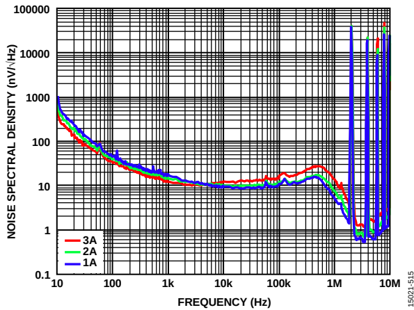
Figure 15. Adaptive Mode Noise Spectral Density vs. Frequency at various Load Currents, V_{PVIN1} = V_{PVIN2} = 3.7\text{ V} , V_{PVOUT1} = 3.3\text{ V} , f_{SW} = 2\text{ MHz} , L = 1.5\text{ }\mu\text{H} , R_C = 23.7\text{ k}\Omega , C_C = 1\text{ nF} , C_{CP} = 10\text{ pF} , C_{PVOUT1} = 22\text{ }\mu\text{F}
