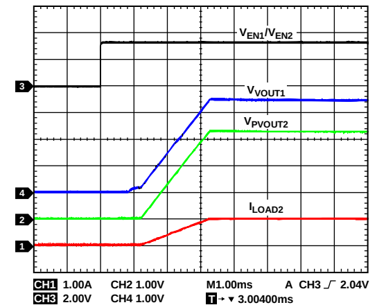
Figure 31. Adaptive Mode Startup, V_{PVOUT2} = 3.3V , I_{LOAD2} = 1A ( V_{EN2} is the EN2 voltage.)
