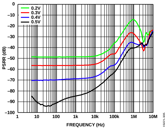
Figure 10. LDO PSRR vs. Frequency, V_{PVOUT2} = 1.3\text{ V} , I_{LOAD2} = 1\text{ A} at Various LDO Headroom Voltages
