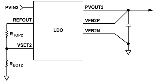
Figure 45. LDO Adjustable Output Voltage Configuration
