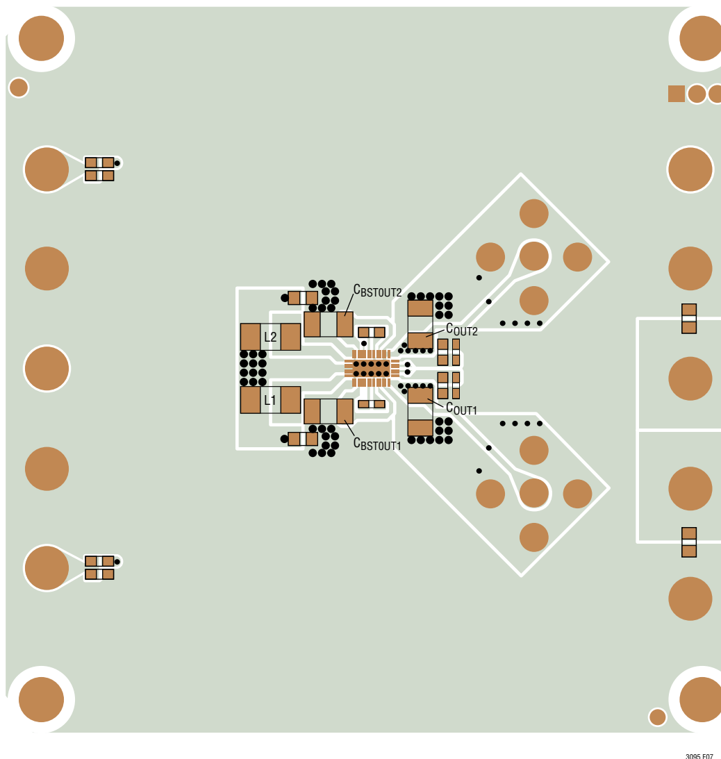
Figure 7. Example PCB Layout, Top Layer (Demo Board DC2270A)
