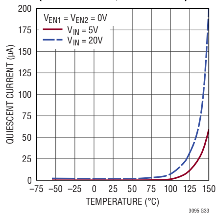
Quiescent Current in Shutdown (Both Channels, Boost + LDO)
