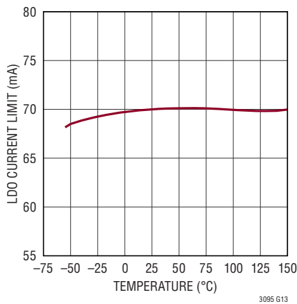
LDO Current Limit
