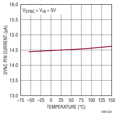
SYNC Pin Current
