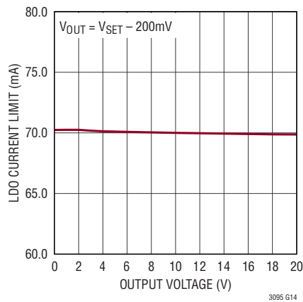
LDO Current Limit
