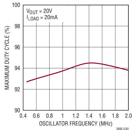
Maximum Duty Cycle
