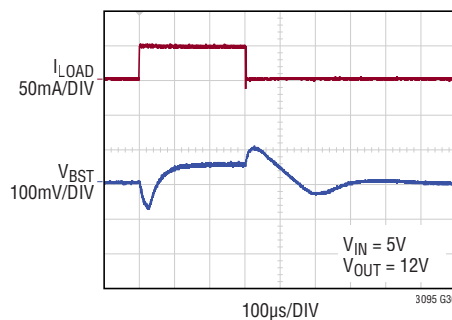
Boost Transient Response
