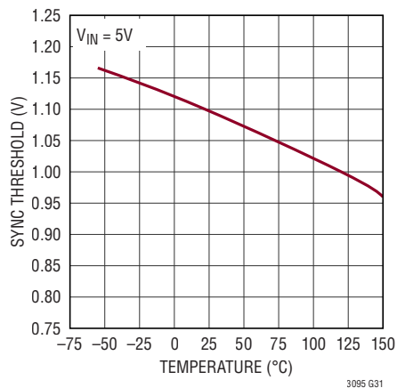
SYNC Threshold
