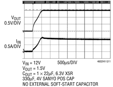
Start-Up, I_{OUT} = 6A (Resistive Load)
