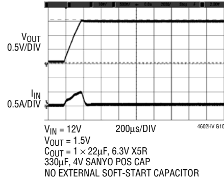
Start-Up, I_{OUT} = 0A
