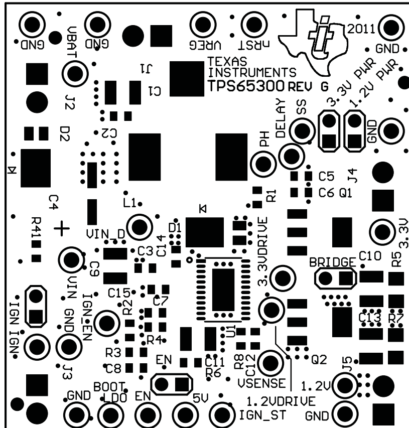
Figure 7. Top Assembly Layer
