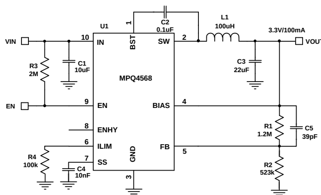
Figure 8 — Detailed Application Schematic
