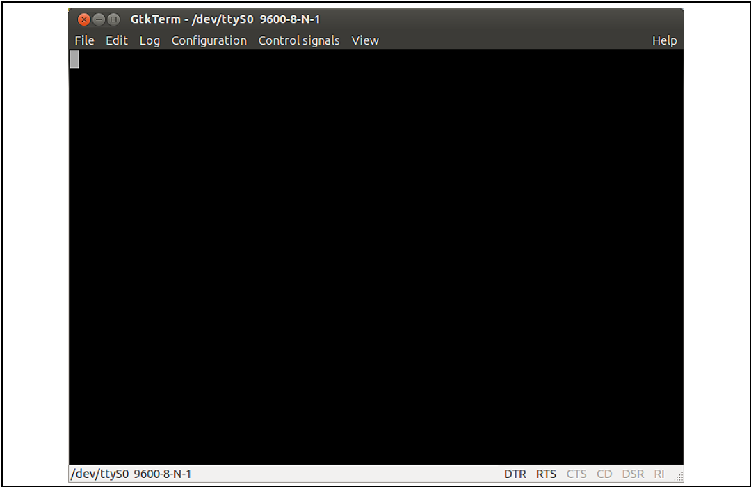
Figure 3. GtkTerm screen
