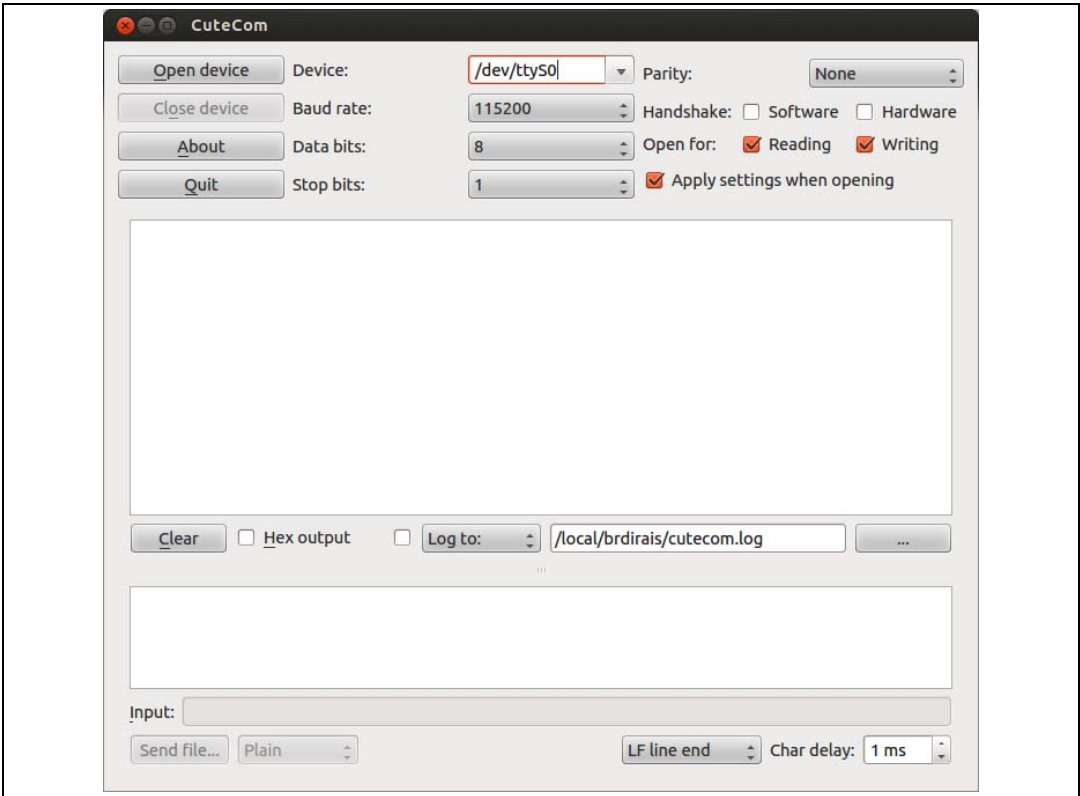
Figure 4. CuteCom screen
