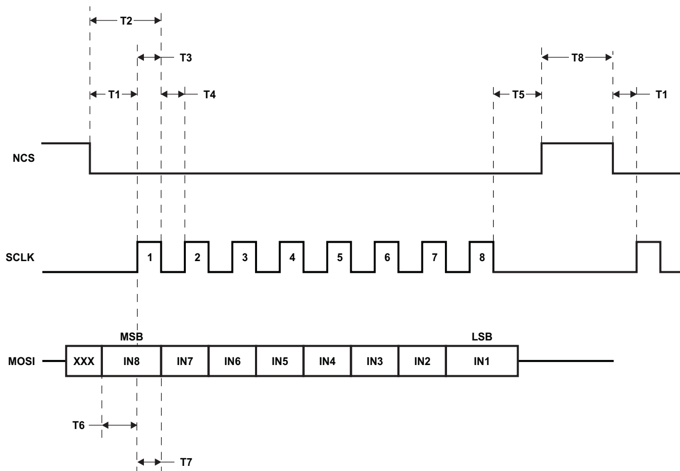
Figure 1. Serial Communications
