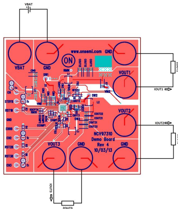
Figure 5. NCV97310 Board Connections
