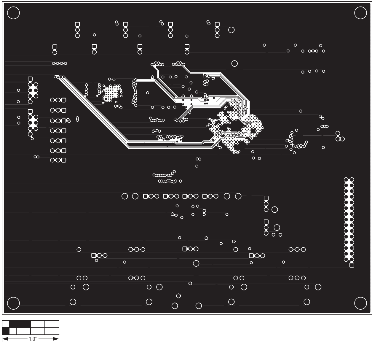
Figure 16. MAX11103 EV Kit PCB Layout—Layer 9
