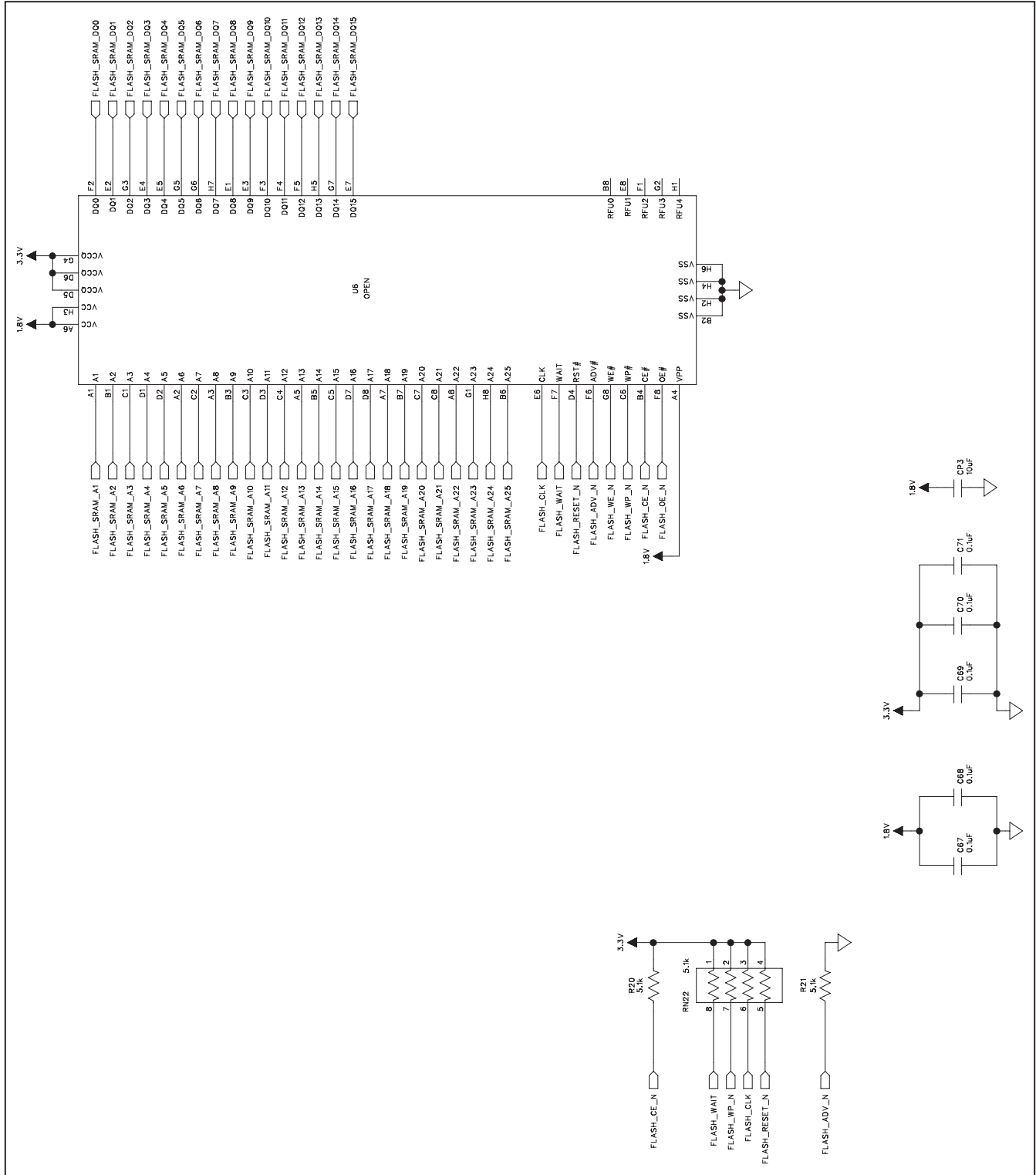
Figure 6i. MAX11103 EV Kit Schematic (Sheet 9 of 12)
