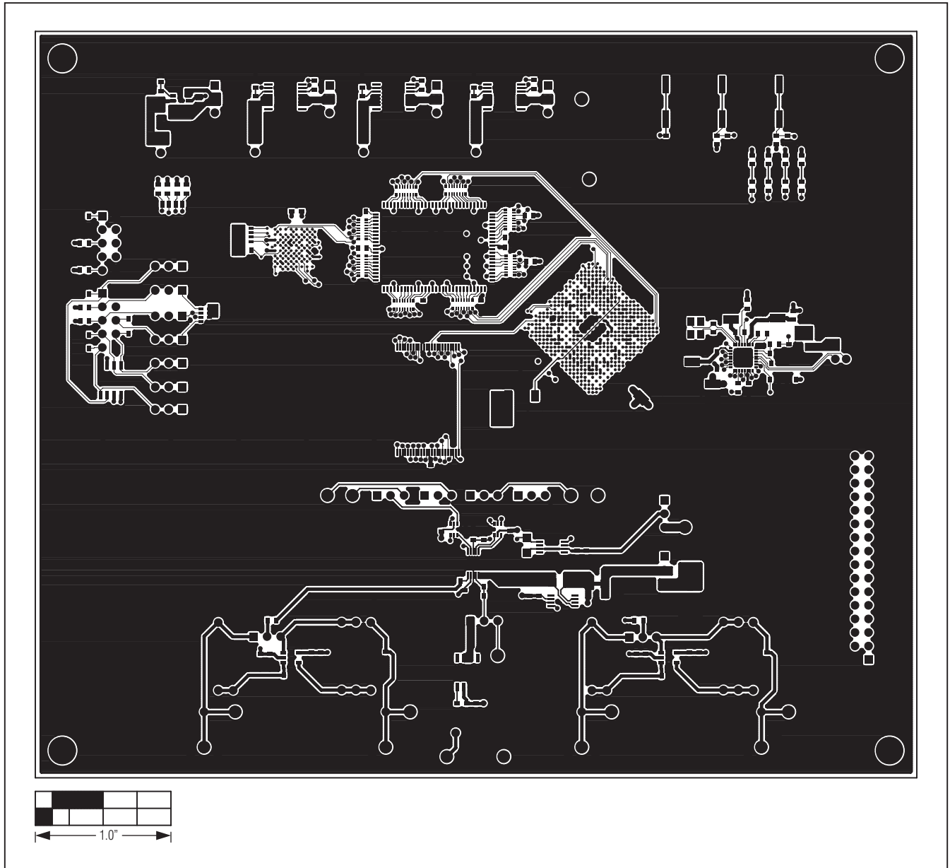
Figure 8. MAX11103 EV Kit PCB Layout—Component Side
