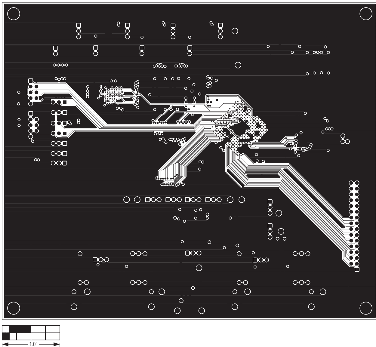
Figure 10. MAX11103 EV Kit PCB Layout—Layer 3
