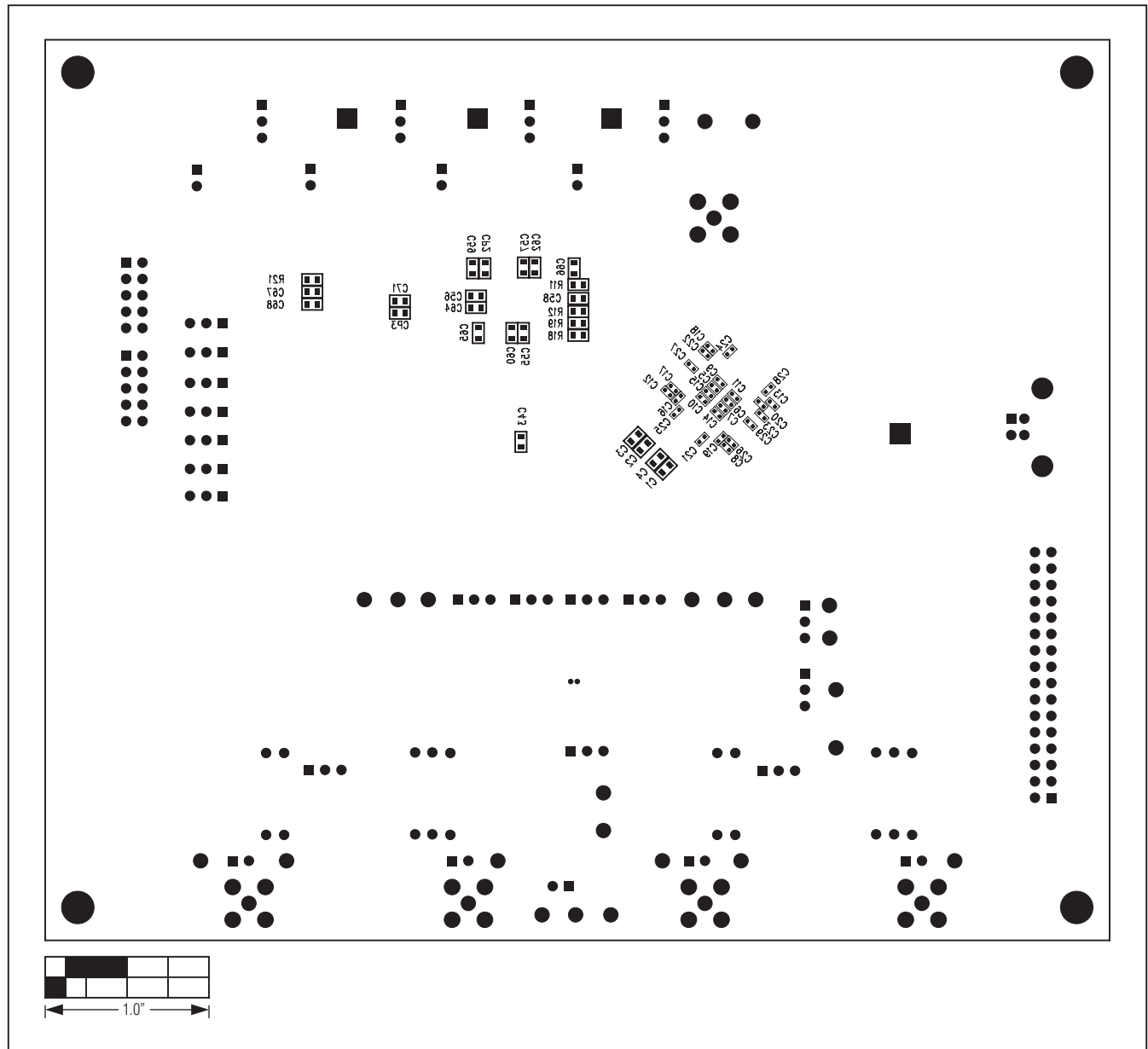
Figure 20. MAX11103 EV Kit Component Placement Guide—Bottom
