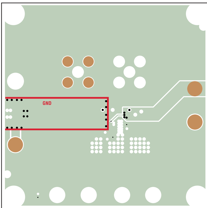
Figure 3. Layer 3 of DC2624A
