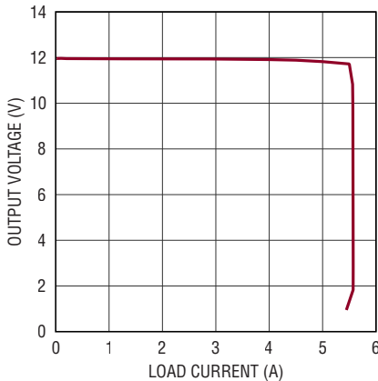
V_{OUT} vs I_{OUT} (CV/CC)
