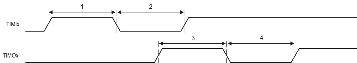
Figure 7-62 Timer Timing
