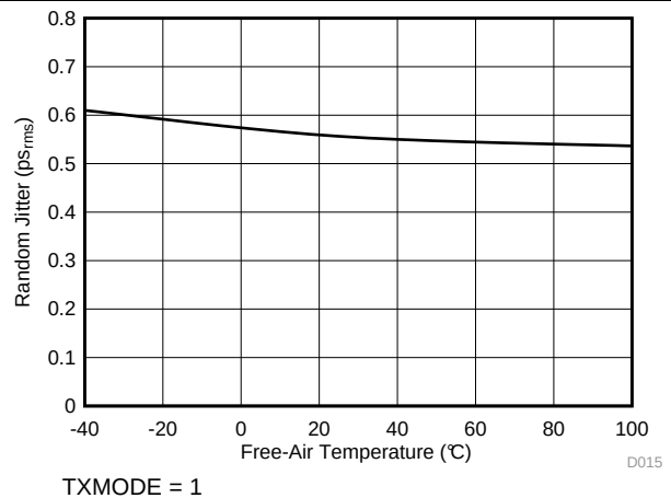
Figure 7. TX Random Jitter vs Temperature
