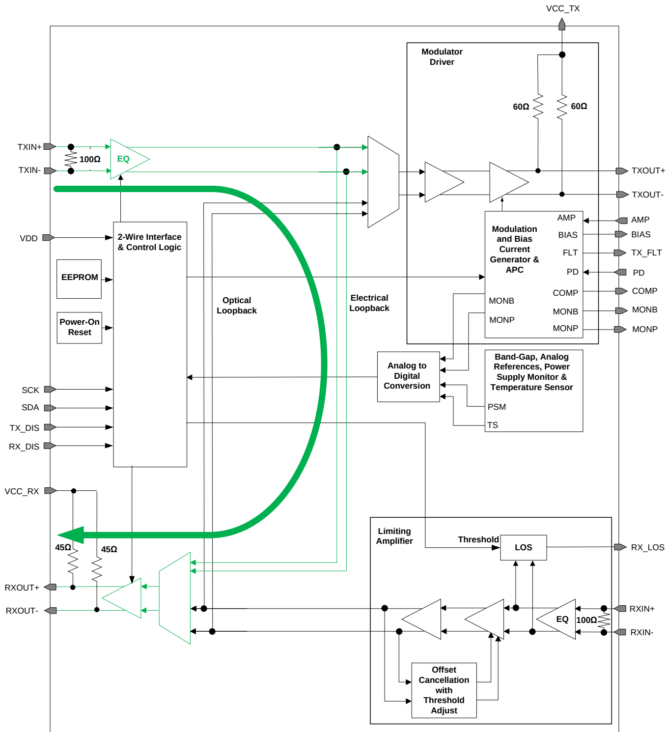
Figure 35. Electrical Loopback
