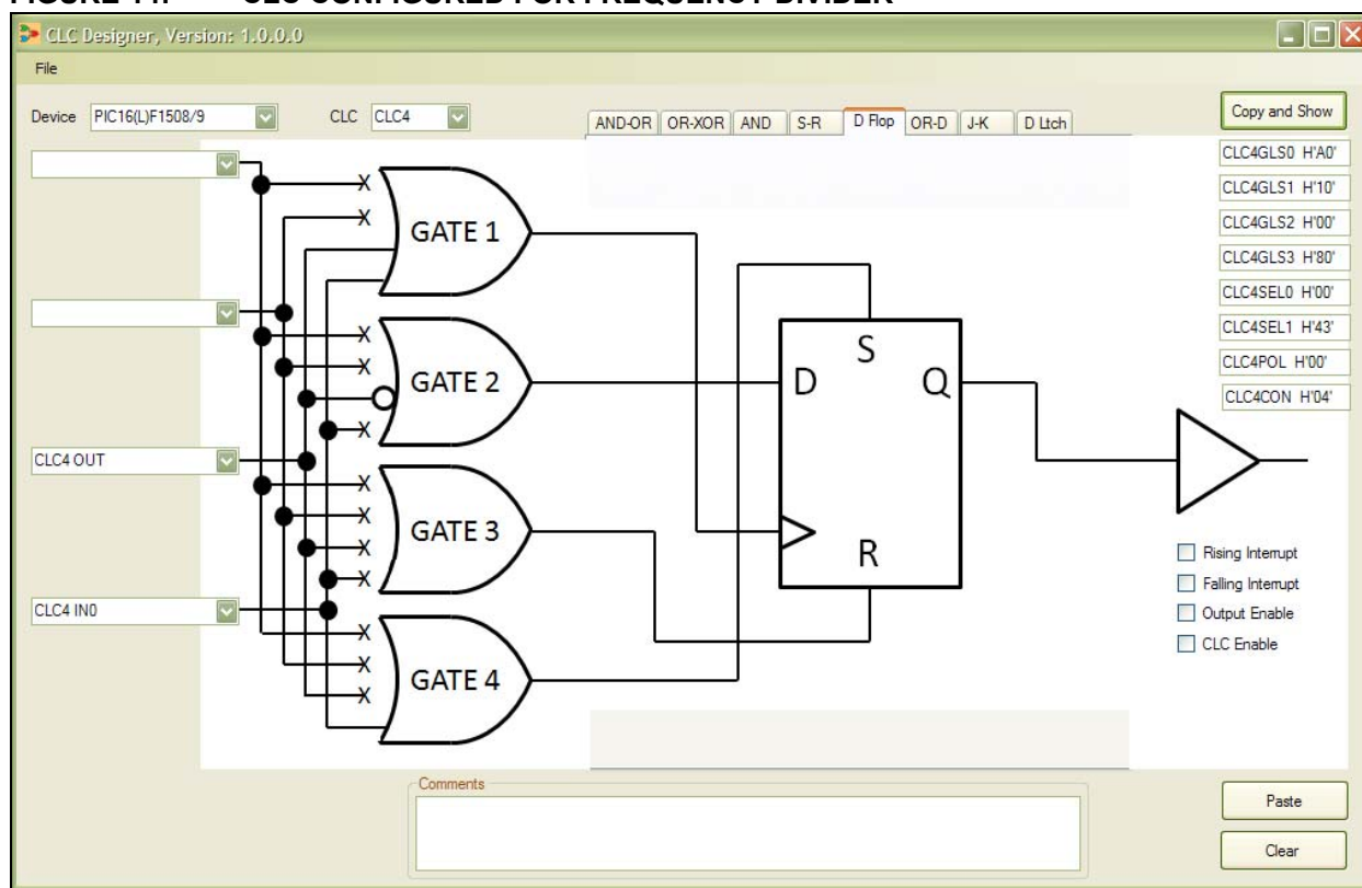
FIGURE 14: CLC CONFIGURED FOR FREQUENCY DIVIDER
