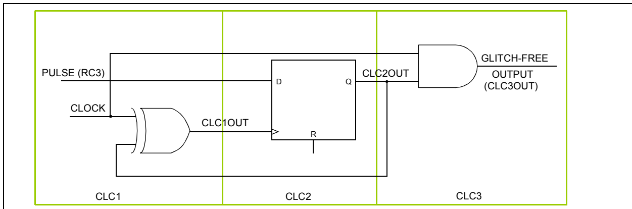
FIGURE 31: CLC SETUP FOR GLITCH-FREE SIGNAL
