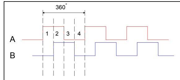
FIGURE 17: QUADRATURE-ENCODED SIGNAL
