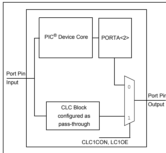
FIGURE 32: BLOCK DIAGRAM
