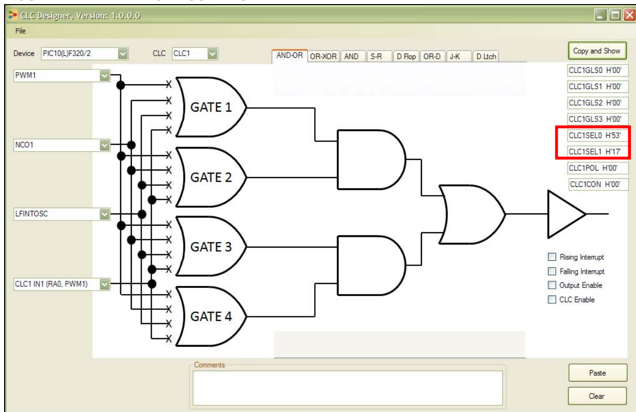
FIGURE 1: CLC CONFIGURATION
