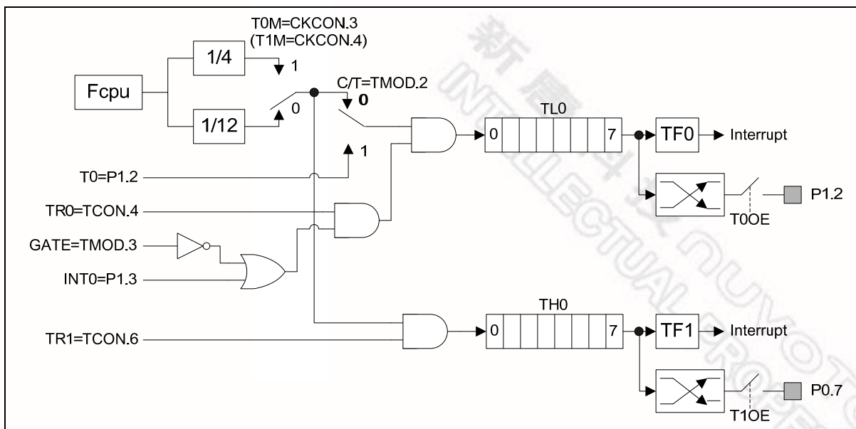
Figure 13-4: Timer/Counter Mode 3
