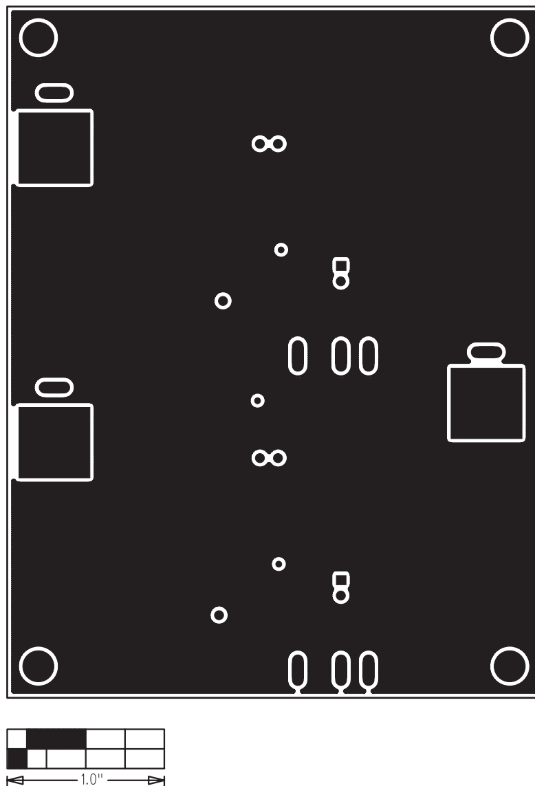
Figure 6. MAX8555A EV Kit PC Layout—Ground Layer (Layer 4)
