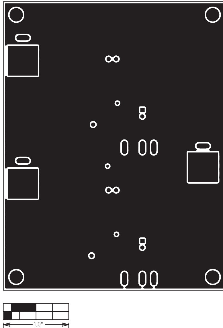
Figure 4. MAX8555A EV Kit PC Layout—Ground Layer (Layer 2)
