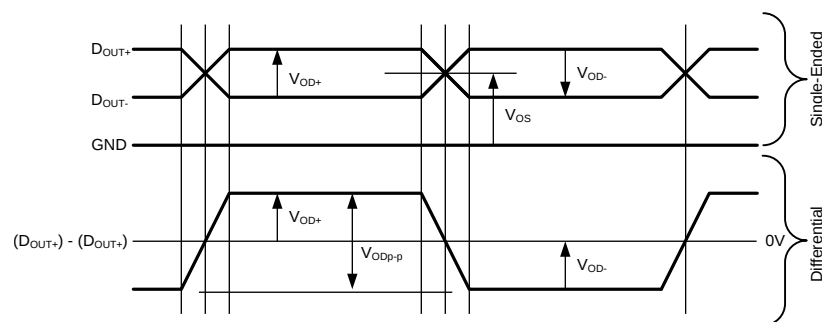
Figure 2. Serializer Output Waveforms
