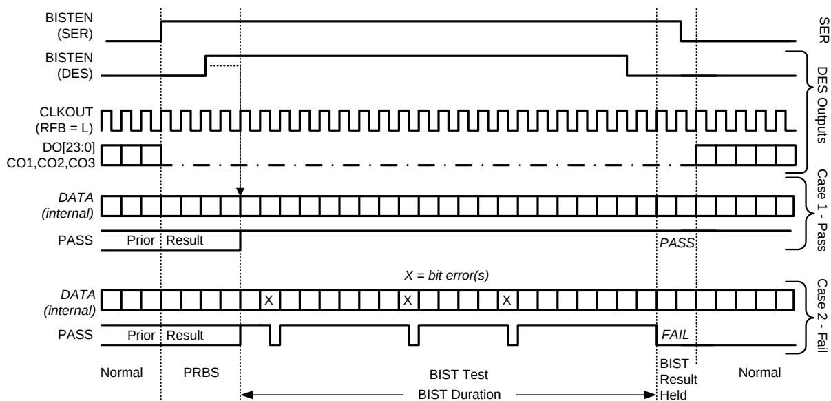
Figure 29. BIST Waveforms
