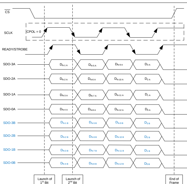
Figure 61. CRT-Q-DDR Protocol
