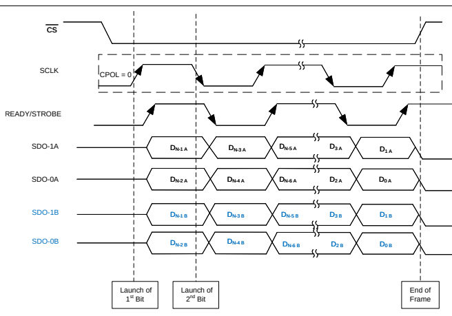
Figure 59. CRT-D-DDR Protocol
