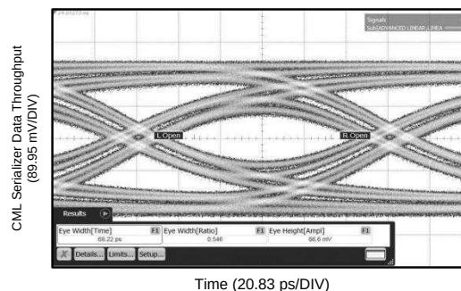
Figure 18. TL = 5-Meter 30-AWG 100 \Omega Twin-Axial Cable, DS80PCI810 CHA_0, 8 Gbps
