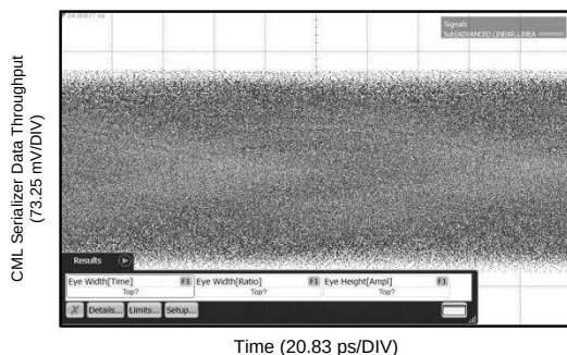
Figure 17. TL = 5-Meter 30-AWG 100 \Omega Twin-Axial Cable, No Repeater, 8 Gbps
