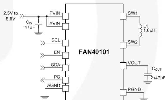
Figure 1. Typical Application
