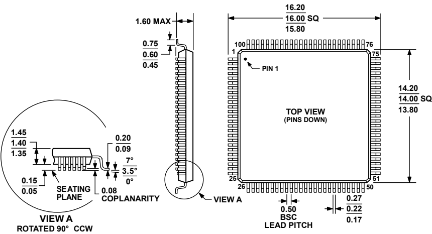
COMPLIANT TO JEDEC STANDARDS MS-026-BED Figure 36. 100-Lead Low Profile Quad Flat Package [LQFP] (ST-100) Dimensions shown in millimeters
