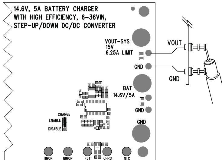
Figure 2. Proper Noise Measurement Setup
